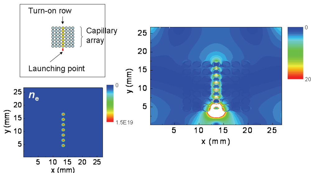
Fig. 4. 2D Wave propagation along a chain structure composed of columnar plasmas at 6.2 GHz. Inset figures show assumed configuration with assumed n_e profile in shape of 0th order Bessel function with peak density of 1.5 \times 10^{13} \text{ cm}^{-3} .
