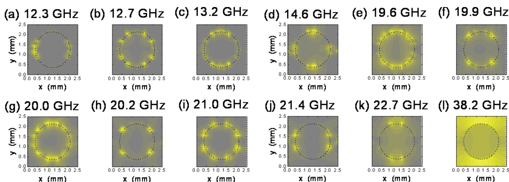
Fig. 9. Calculated profiles of electric fields normalized in amplitude in case of k_x a/2\pi = 0.25 and k_y = 0 . Parameters used are similar to Fig. 8. (Sakai & Tachibana, 2007)
