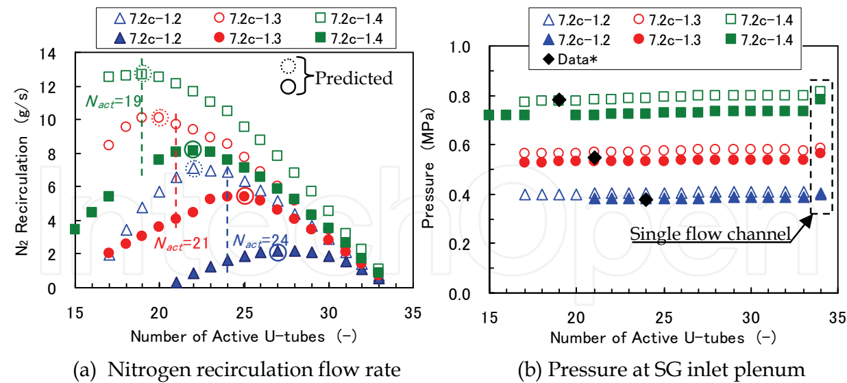
Fig. 10. Effects of number of active U-tubes as calculation parameter; open: plenum volume of 0.02 m³; closed: plenum volume of 0.05 m³; N_{act} : observed number of active U-tubes*; *Data: Noel & Deruaz (1994)
