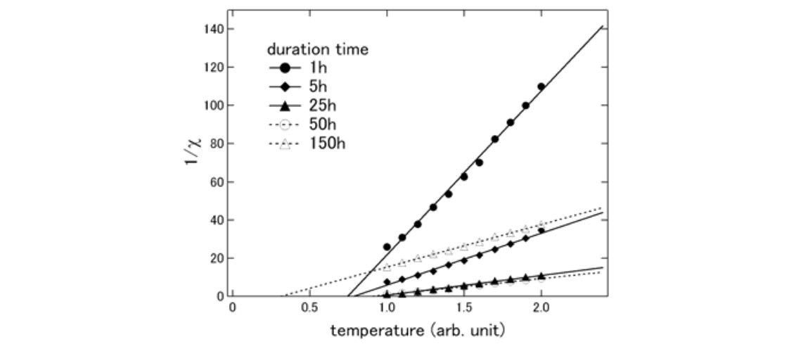
Fig. 33. Temperature dependence of inverse of calculated magnetic susceptibility 1/\chi for each duration time.
