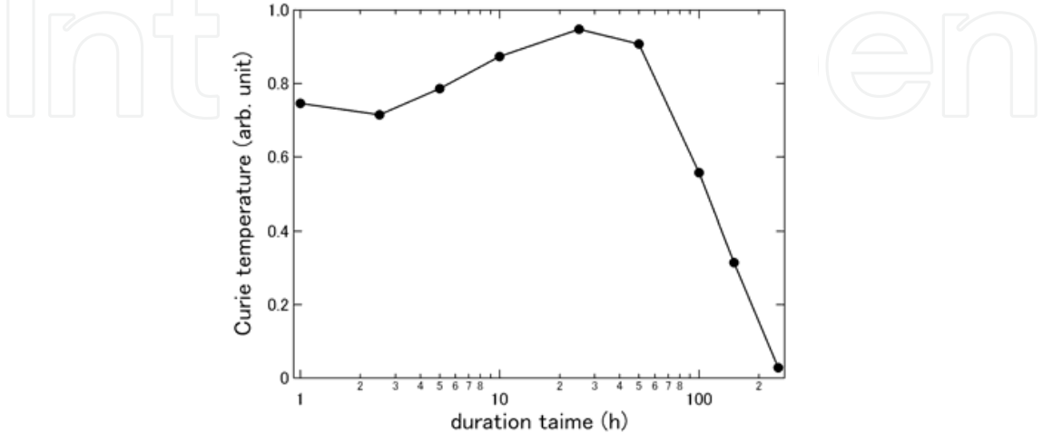
Fig. 34. Duration time dependence of Curie temperature.
