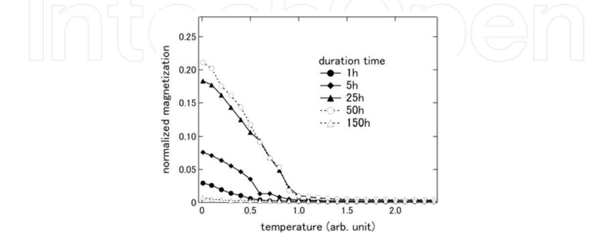
Fig. 31. Temperature dependence of calculated magnetization for each duration time
