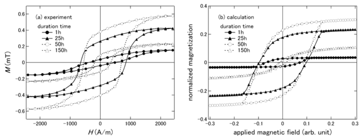
Fig. 28. M-H curves of (a) experiment and (b) calculation for each duration time.
