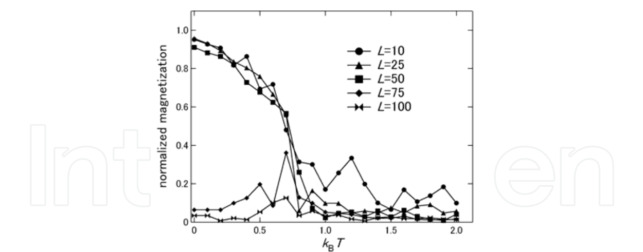
Fig. 5. Temperature dependence of normalized magnetization M for different size square clusters.
