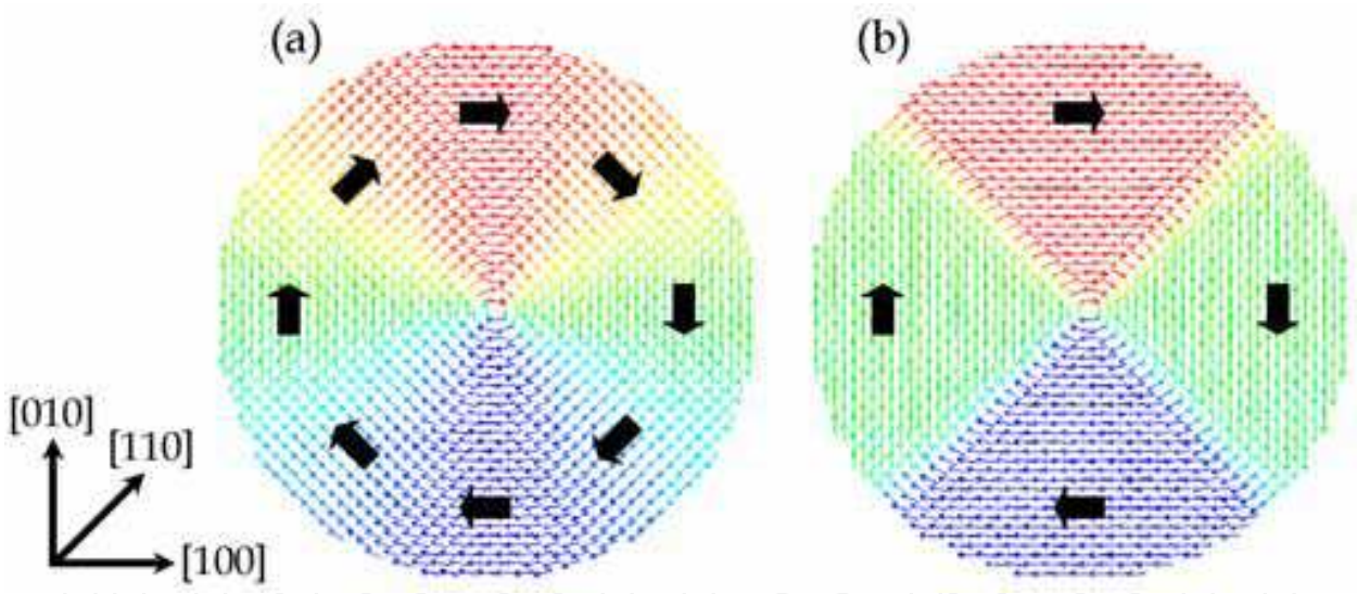
Fig. 11. Spin snapshots for a cylindrical cluster at the lowest temperature using Hamiltonian; (a) H_J+H_D , (b) H_J+H_D+H_{A\_macro} .
