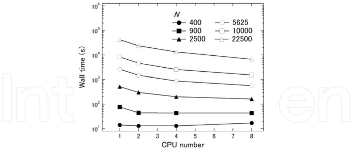
Fig. 3. Wall time during 1000 MCS depending on CPU number for each size cluster ( N=L^2 ).
