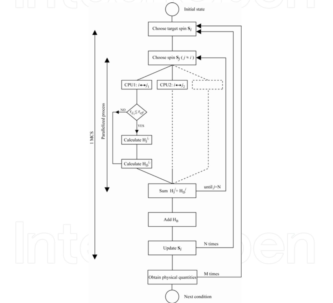
Fig. 2. Flowchart of MC algorithm including parallelized process. The process from “Choose spin S_j ” to “Sum H_j + H_D ” is parallelized in this algorithm. The process from “Choose spin S_i ” to “Update S_i ” is repeating until spin total number N and it is called 1MCS. Figure 6 shows spin snapshots for the different size square clusters with the one side length of L=10, 50, 75 , respectively at lowest temperature. It is clearly seen that the closure domain structure of spin system actually appears for the cluster with L=75 .
