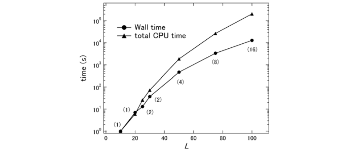
Fig. 4. Total CPU time and wall time on calculation at a fixed temperature for each size cluster. Numbers in brackets ( ) show the CPU numbers for parallel calculation.
