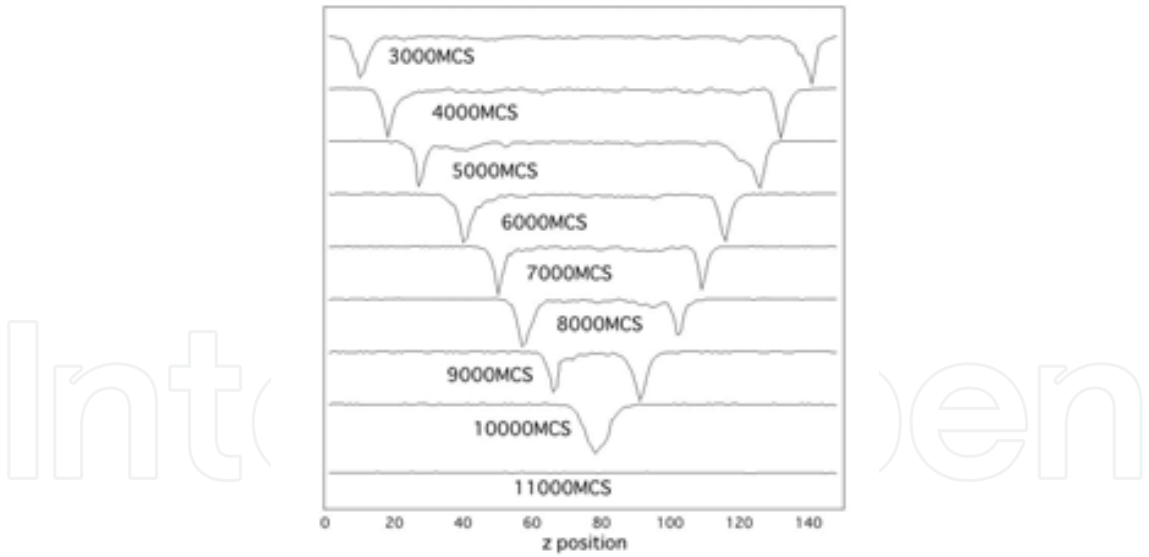
Fig. 22. Average of absolute value of S_z at each z position at each increasing time elapse, respectively. Each dip shows the DW position.
