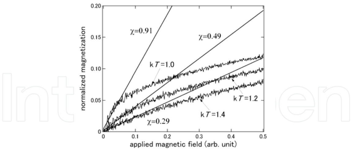
Fig. 32. Example of calculation for magnetic susceptibility \chi from M-H curve at each temperature for the duration time of 25h.
