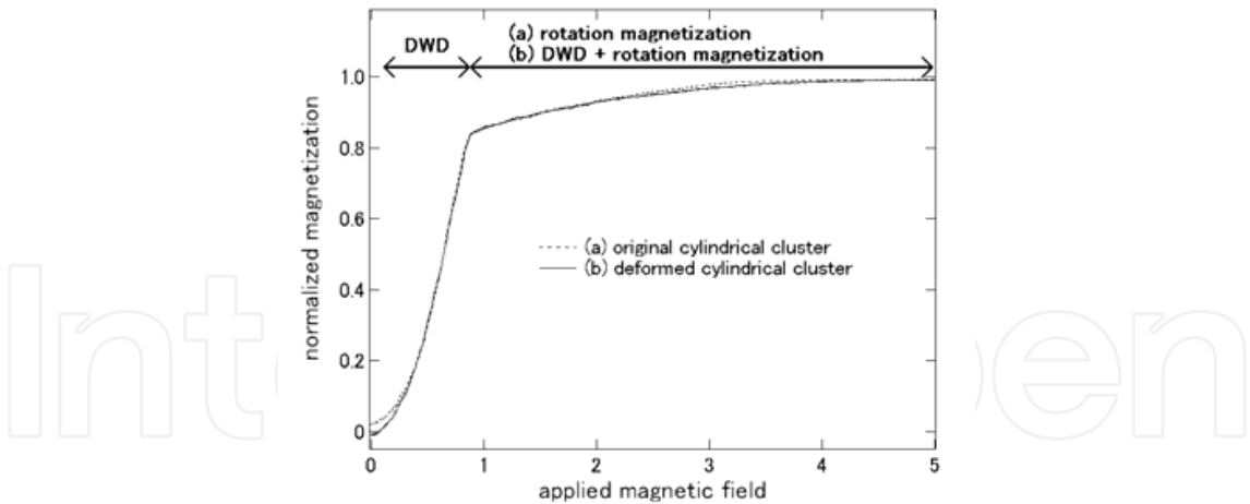
Fig. 16. Magnetizations as a function of applied magnetic fields along the [110] direction for (a) the original cylindrical cluster and (b) the deformed cylindrical cluster using H_2= H_J+H_D+H_{A\_micro}+H_B . Note that parameter A in (4b) is set to A =10 .
