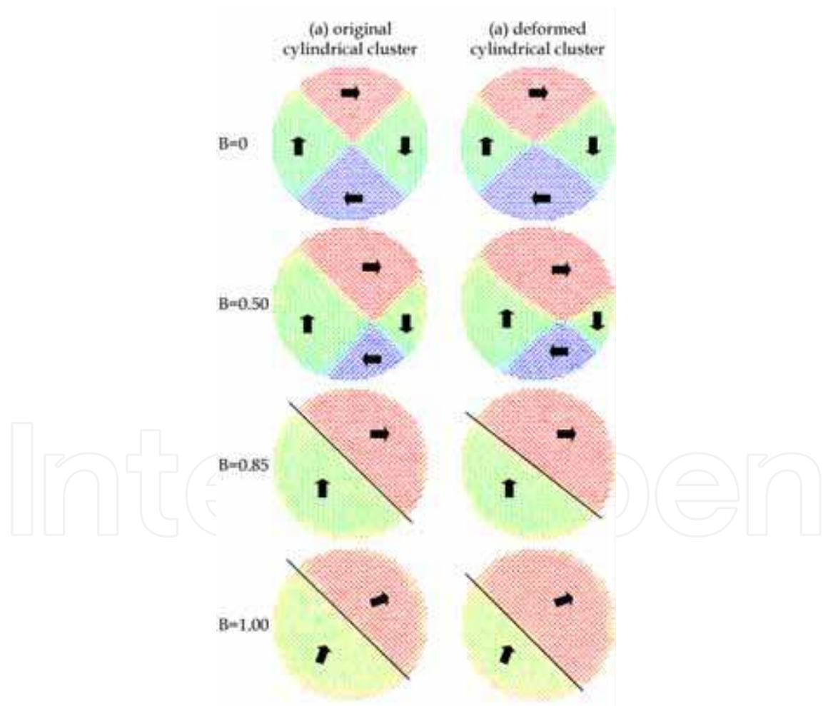
Fig. 15. Spin snapshots on magnetization processes for (a) the original cylindrical cluster and (b) the deformed cylindrical cluster elongated 1.01 times along the [010] direction, when magnetic fields were applied along the [110] direction. Note that parameter A in (4b) is set to A=10 .
