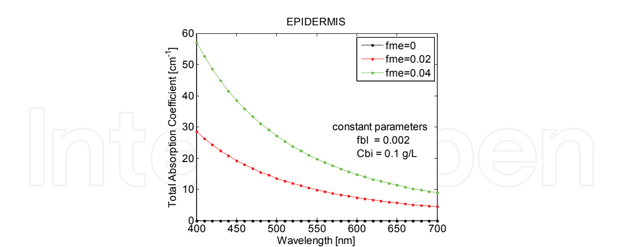
Fig. 3. Absorption coefficient of epidermis for the optical model as the volume fraction of melanosomes, f_{me} , is varied.
