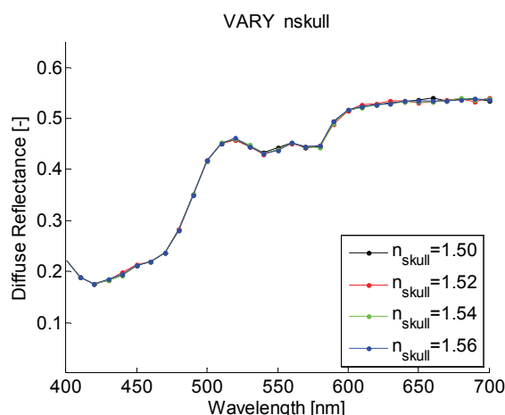
Fig. 5. Diffuse reflectance spectra of neonatal skin when the refractive index of skull is varied while the remaining parameters ( C_{bi} = 0.1 g/L, f_{bl} = 0.002 , f_{me} = 0.02 and n_{fat} = 1.44 ) of the model are kept constant.
