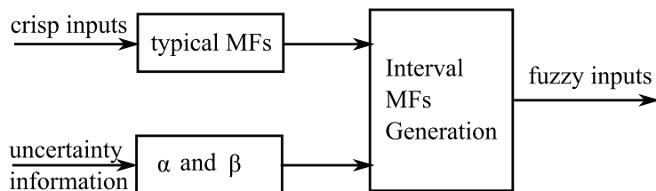
Fig. 3. The interval membership functions(MFs) generation
