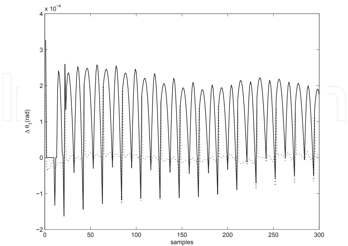
Fig. 10. The angle error of \theta_1 by typical FLS(solid line) and EFLS(dot line)
