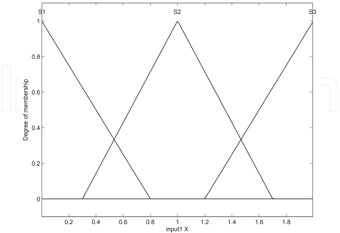
Fig. 8. The fuzzy membership functions of input X
