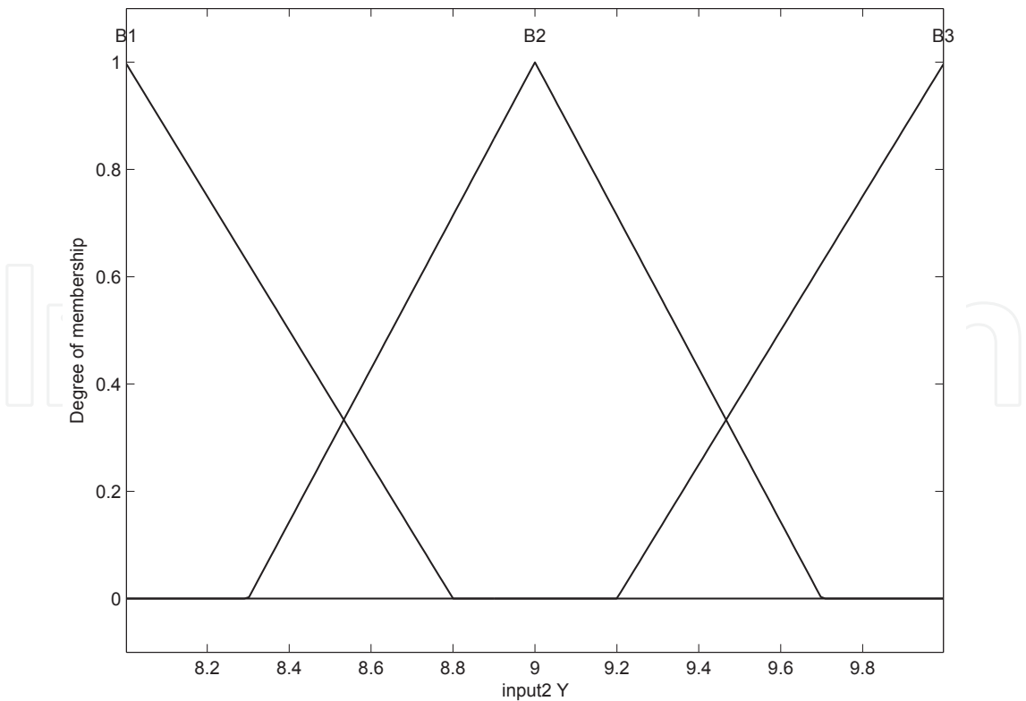
Fig. 9. The fuzzy membership functions of input Y
