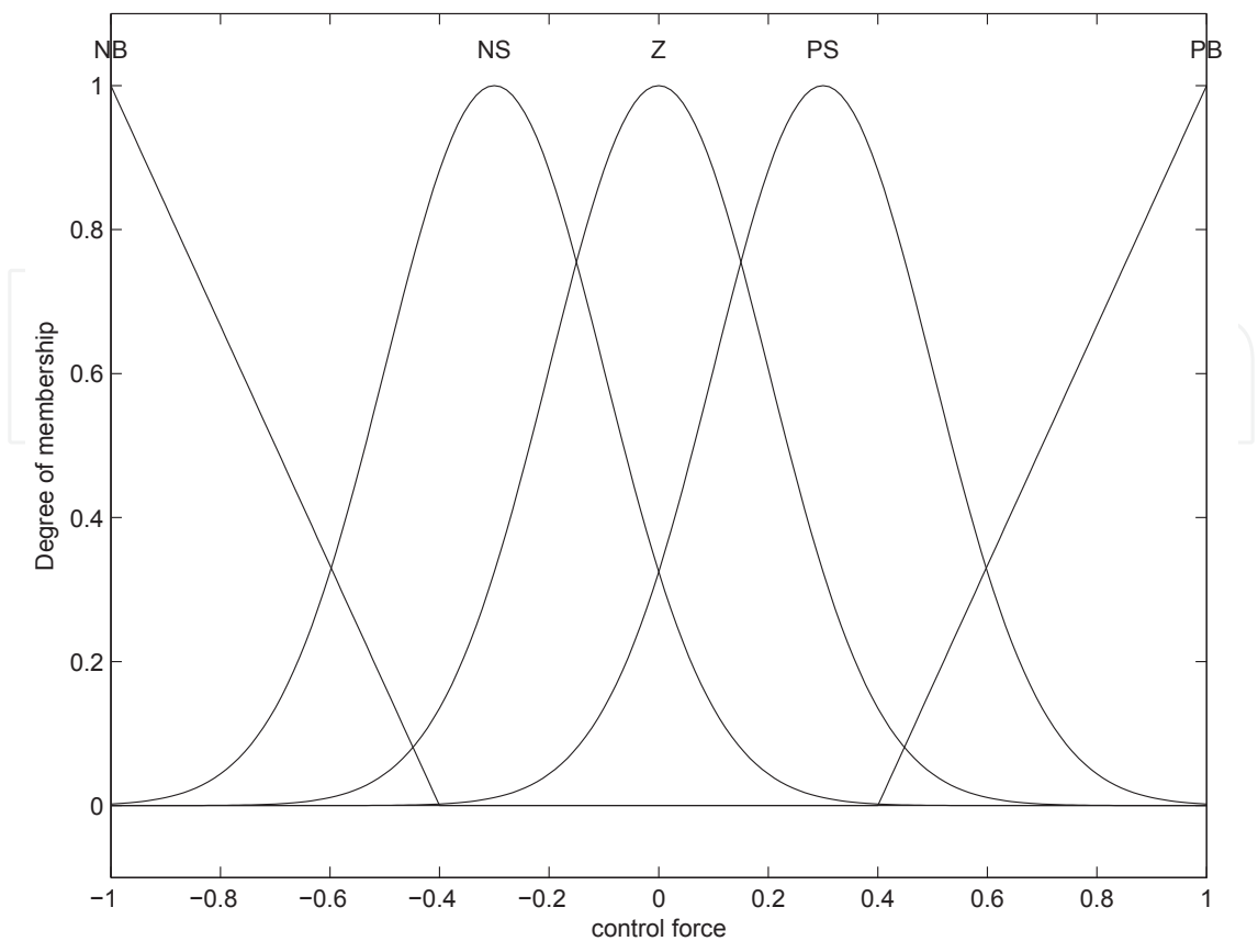
Fig. 16. Membership functions of control forces, f_a
