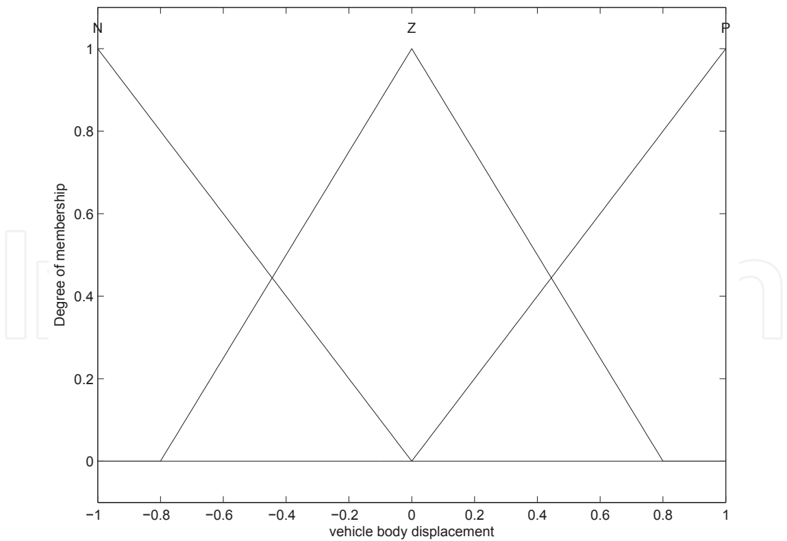
(b) MFs of displacements of the vehicle body, z_b
