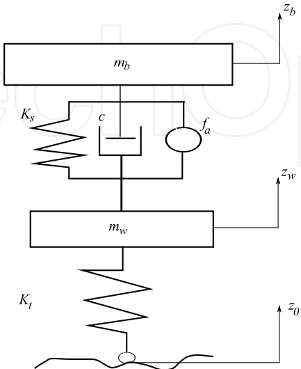
Fig. 14. The quarter vehicle active suspension system
