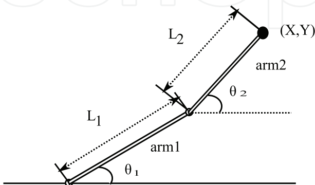
Fig. 7. The two-joint robotic arm with two angles
