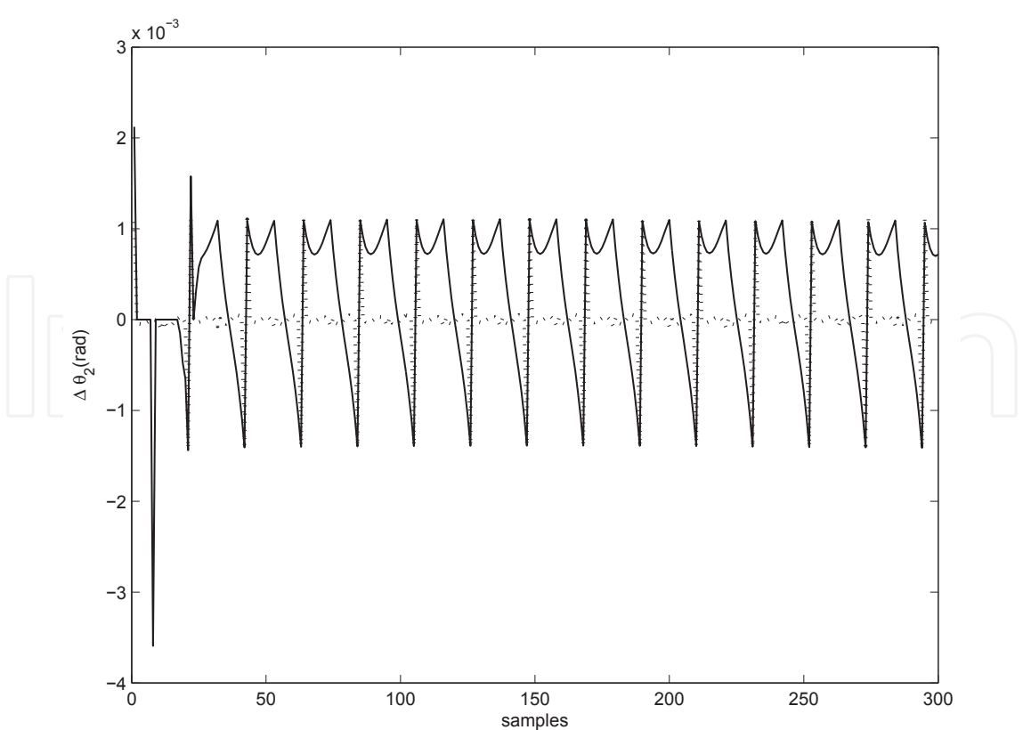
Fig. 11. The angle error of \theta_2 by typical FLS(solid line) and EFLS(dot line)
