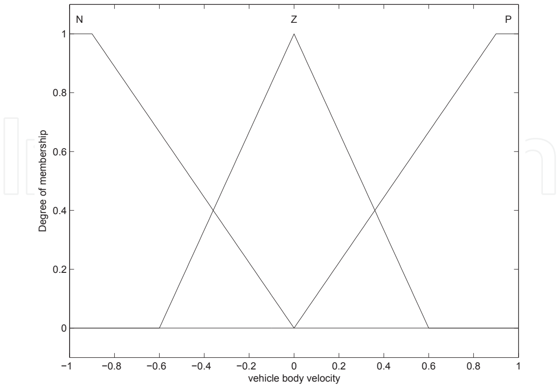
(a) Membership functions of the vehicle body velocities, \dot{z}_b
