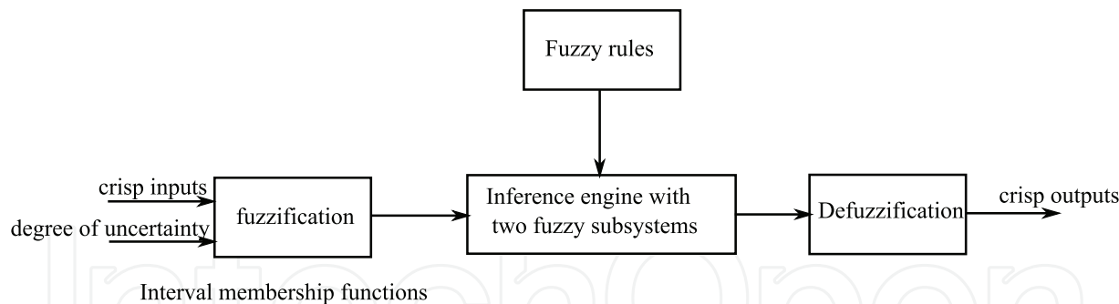
Fig. 2. The framework of interval fuzzy logic system
