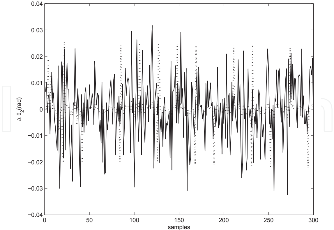
Fig. 13. The angle error of \theta_2 by type-1 FLS(solid line) and EFLS(dot line) with random noise
