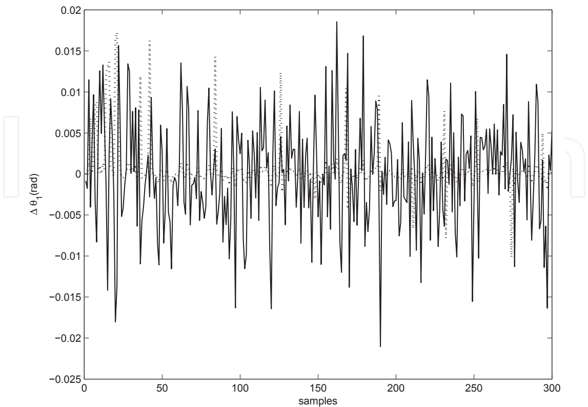
Fig. 12. The angle error of \theta_1 by type-1 FLS(solid line) and EFLS(dot line) with random noise
