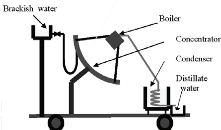
Fig. 15. Experimental device.
