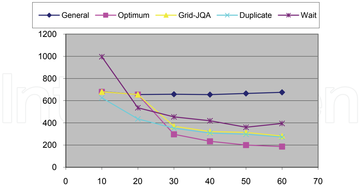
Fig. 12. Simulation for random request (1000-6000) and random capabilities (1000-6000)
