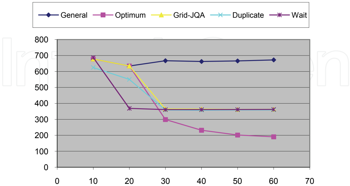
Fig. 11. 1000 cpu cycle request with threshold is 2
