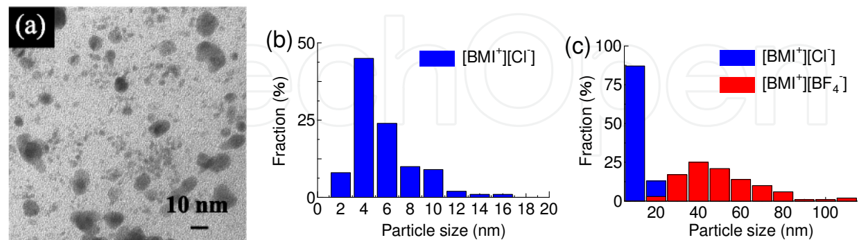
Fig. 13. (a) TEM images of the Au nanoparticles synthesized using the ionic liquid [BMI+][Cl−]. P_{Ar} = 60 Pa, I_D = 1 mA, t = 15 min. (b) Particle size distribution of the Au nanoparticles synthesized in the ionic liquid [BMI+][Cl−] estimated by TEM image in Fig. 13(a). (c) Comparison of the particle size distributions between the cases of [BMI+][Cl−] and [BMI+][BF 4 −].
