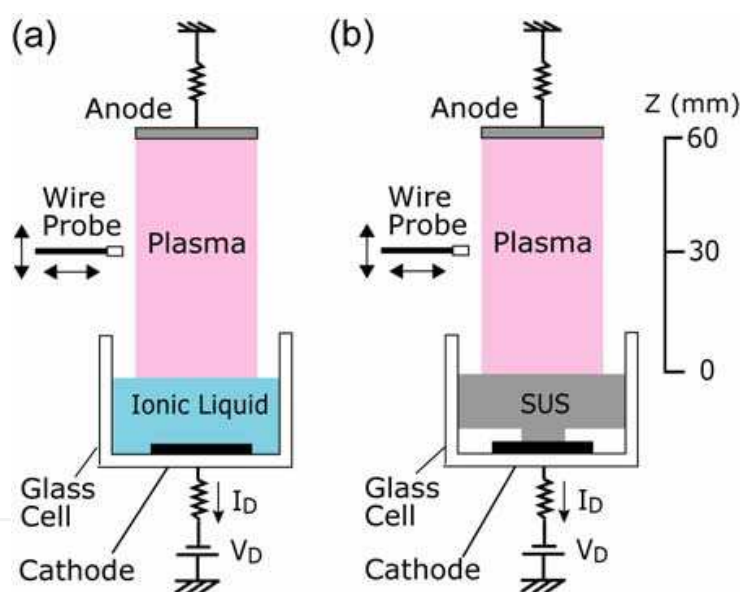
Fig. 1. Schematic diagrams of experimental setup for DC discharge plasmas, where the cathode is set in the glass cell, and is (a) the ionic liquid and (b) the SUS plate. The anode is located at the top of the gas plasma region. These configurations are defined as A-mode.
