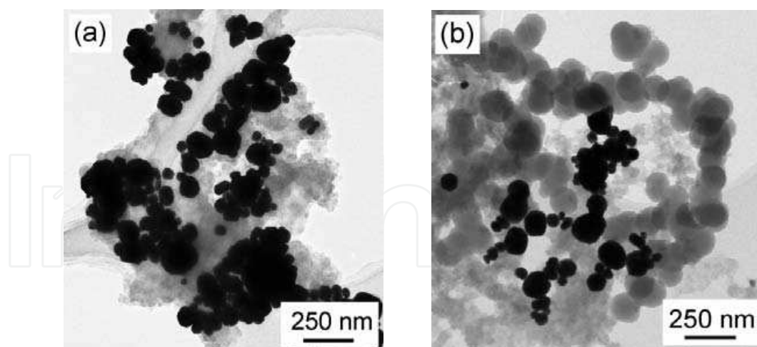
Fig. 11. TEM images of the Au nanoparticles synthesized in (a) A-mode and (b) B-mode. P_{Ar} = 60 Pa, I_D = 1 mA, t = 40 min.
