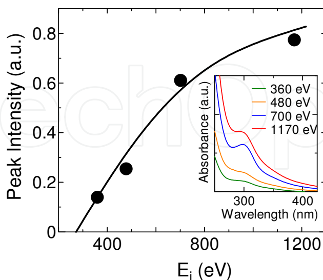
Fig. 9. Peak intensity of UV-Vis absorption spectra of the ionic liquid ( [\text{BMI}^+][\text{BF}_4^-] ) at 297 nm as a function of the ion irradiation energy E_i in A-mode. I_D = 1 \text{ mA} , t = 2 \text{ min} . Inset is the absorption spectra with E_i as a parameter.
