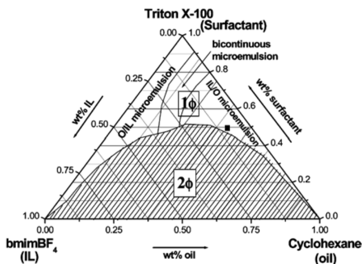
Fig. 1. Ternary phase diagram of [\text{bmim}][\text{BF}_4] /TX-100/cyclohexane at 23^\circ\text{C} . (Reproduced from (Gao et al., 2008) with permission, copyright American Chemical Society, 2008).
