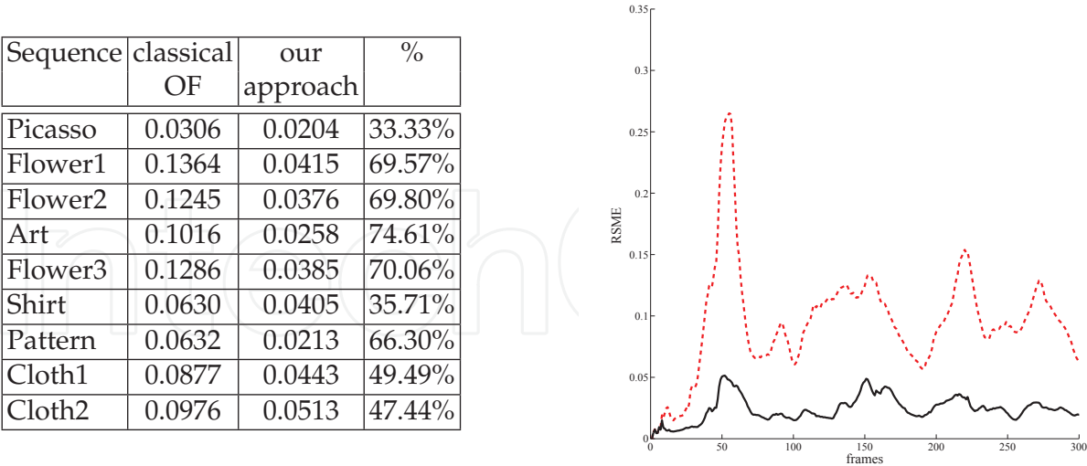
Fig. 5. Left: Comparison of the average RMSE over the entire video sequence with our approach and classical optical flow. Right: Plots of the RMSE between the synthetic frame \hat{\mathcal{I}}_n and the original current frame \mathcal{I}_n with classical optical flow (dashed red) and our method (solid black) for an example sequence.
