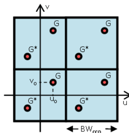
Fig. 2. Distribution of multiple spectra terms G and G^* in the Fourier transform of the sampled version of the hologram h_m(x, y) , recorded by the CCD. This spatial distribution is uniform by using a RW with spatial frequencies u_0 = v_0 = BW_{CCD}/4 .
