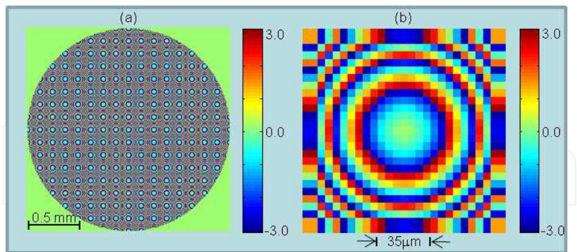
Fig. 14. (a) Wrapped phase modulation of the third test object formed by an array of micro lenses of focal length fL=1.5 mm. (b) Close view of the phase modulation in a single lens of the array.
