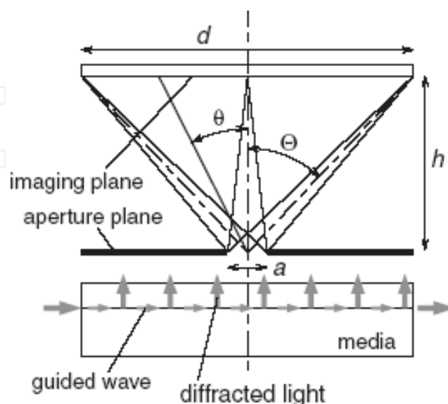
Fig. 8. Schematic view of direct imaging optics.
