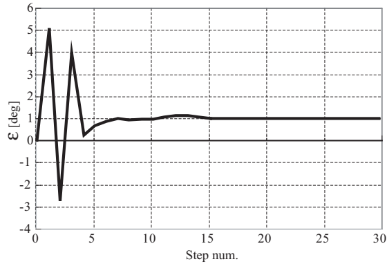
Fig. 16. Alteration of \epsilon in landing position control
