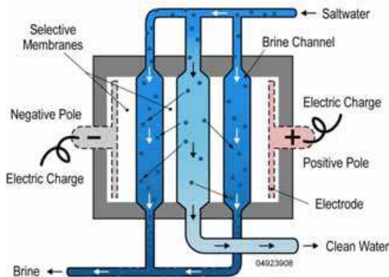
Fig. 9. Diagram of electrodialysis unit (modified from [7])
