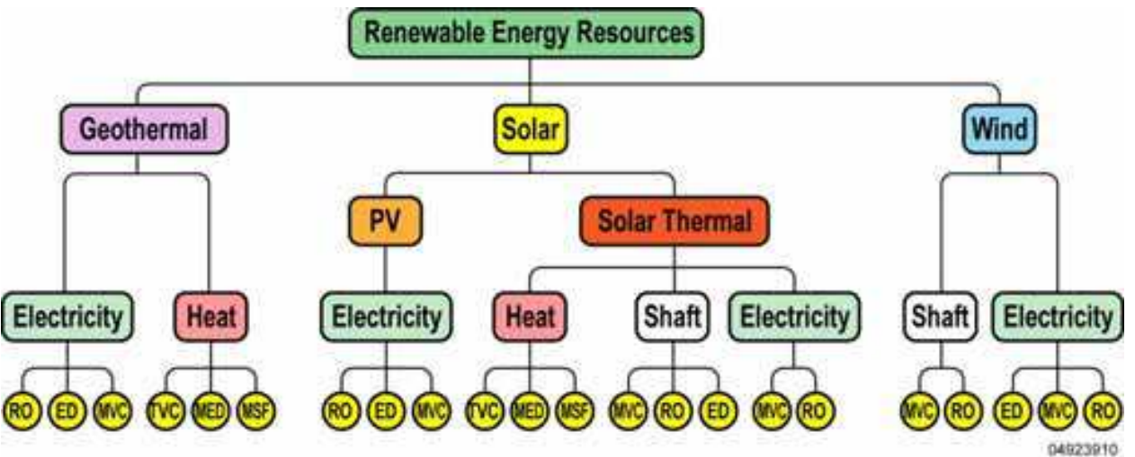
Fig. 10. Possible combinations of renewable energy systems with desalination units. Proper matching of standalone power-supply desalination systems has been recognized as being crucial if the system is to provide a satisfactory supply of power and water at a reasonable cost. Standalone renewable energy systems for electricity supply are now a proven technology and economically promising for remote regions, where connection to the public electric grid is either not cost effective or feasible, and where water scarcity is severe. Solar thermal, solar PV, wind, and geothermal technologies could be used as energy suppliers for desalination systems. Table 1 presents the most promising combinations of renewable energy resources with desalination technologies. According to this table, solar energy –both solar thermal and solar PV– can be used to drive MSF, MED, RO, and ED. Wind energy can drive VC, RO, and ED. Geothermal energy reservoirs with moderate temperature can drive MSF and MED units, while geothermal high pressure reservoirs can be utilized to drive mechanically driven desalination units by shaft power or by producing electricity to drive VC, RO, and ED units.
