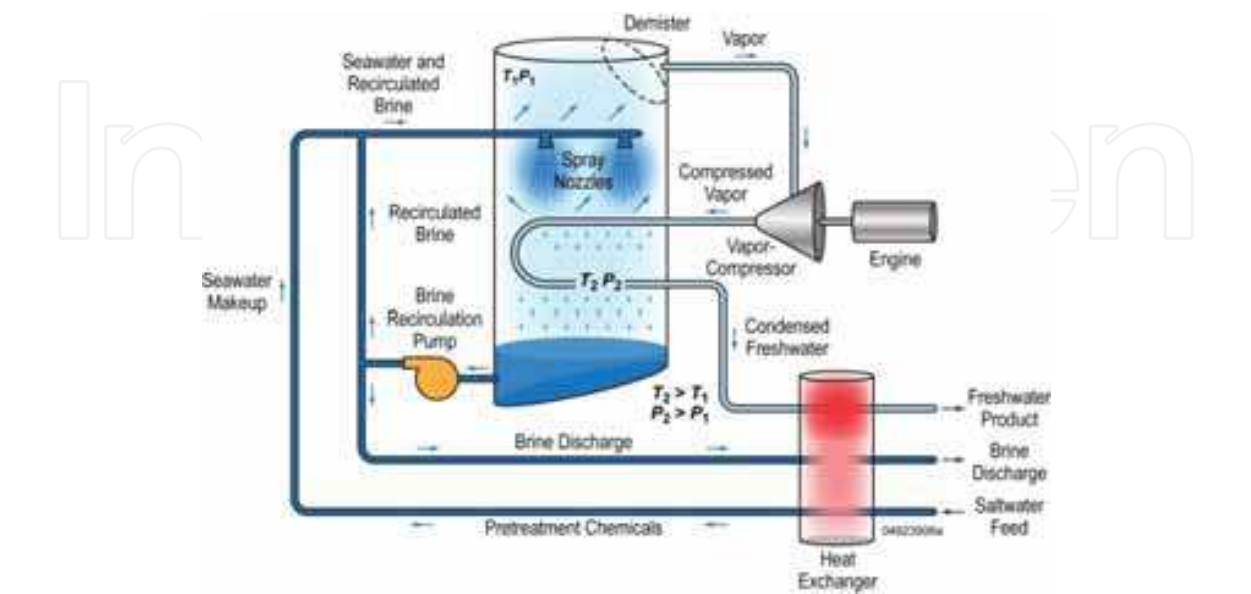
Fig. 6a. Diagram of a mechanical vapor-compression plant.
