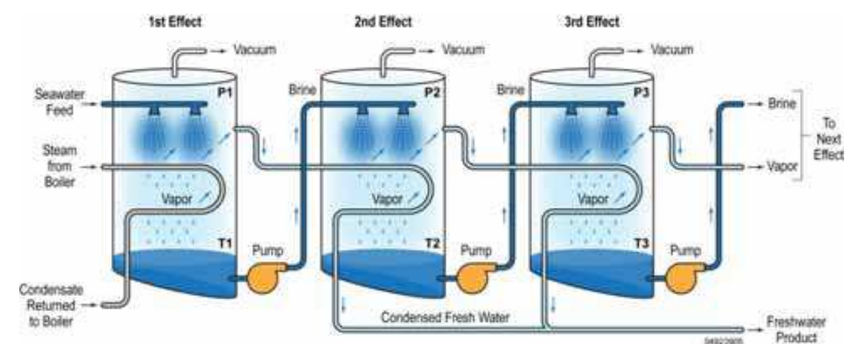
Fig. 5. Diagram of an MED unit (modified from [7])
