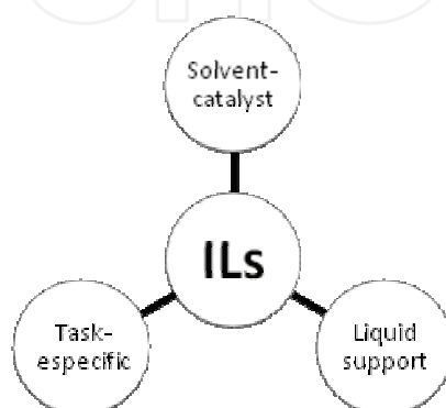
Fig. 2. IL effects in cyclocondensation reactions.
