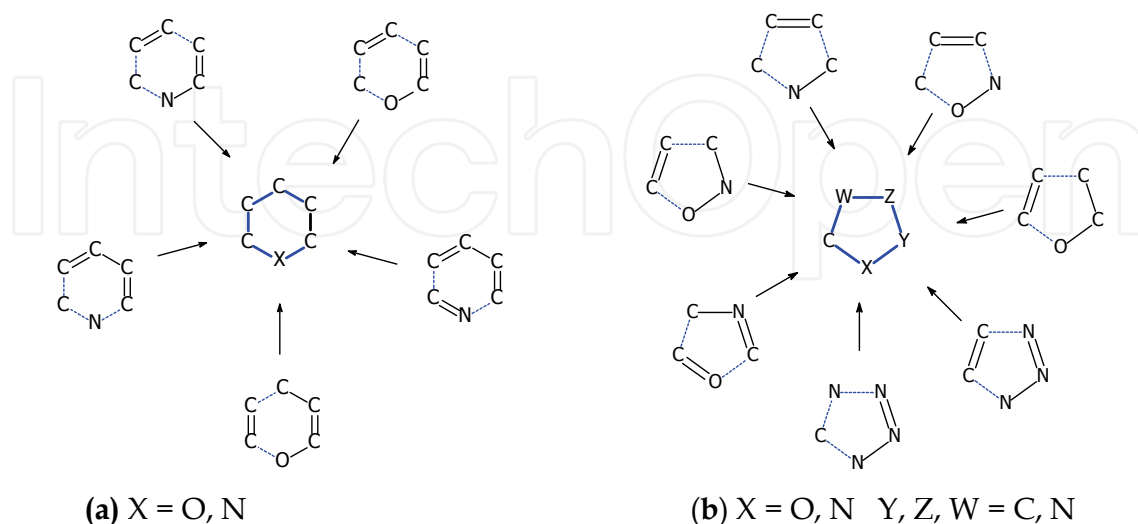
Fig. 4. General 1,3-dipolar cycloaddition and possible combination to form (a) six-membered and (b) five-membered heterocycles.
