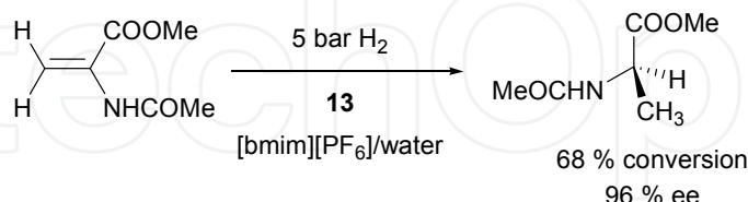
Fig. 25. Hydrogenation of methyl 2-acetamidoacrylate
