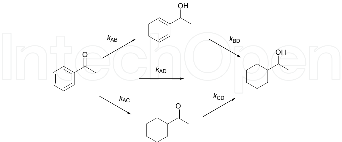
Fig. 5. Kinetic model for the reduction of acetophenone with supported catalysts.
