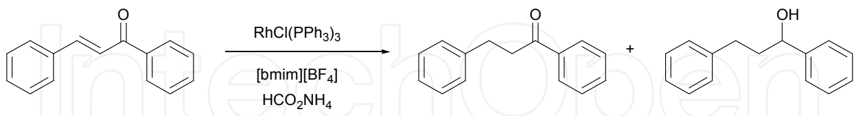
Fig. 63. Hydrogenation of chalcone using Wilkinson’s catalyst
