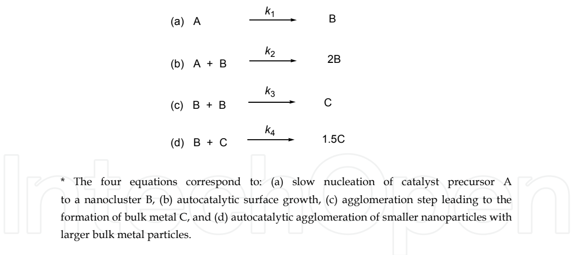
Fig. 6. Four-step mechanism for transition-metal nanocluster nucleation, growth and agglomeration
