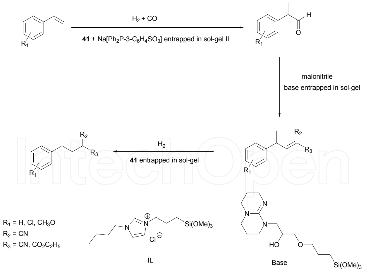
Fig. 66. One-pot multistep process
