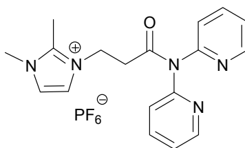
Fig. 37. 2,3-Dimethyl-1-[3- N,N -bis(2-pyridyl)-propylamido]imidazolium hexafluorophosphate
