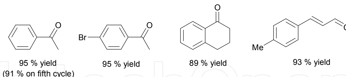
Fig. 61. Carbonyl compounds selectively hydrogenated to alcohols
