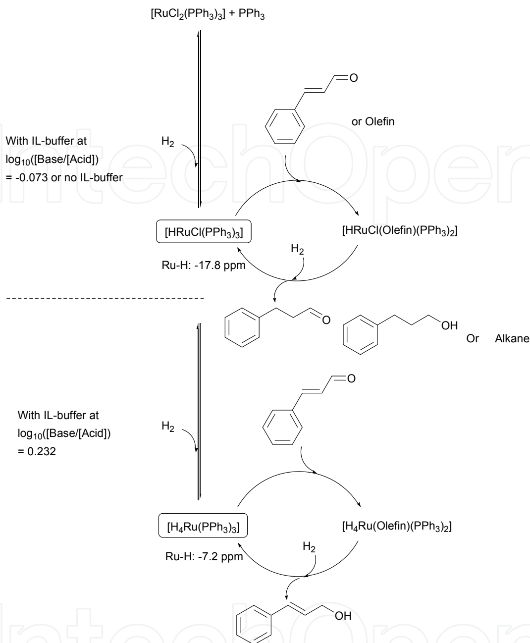
Fig. 64. Hydrogenation using IL-buffers
