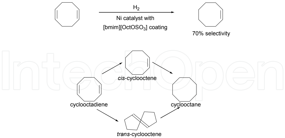
Fig. 65. Hydrogenation of cyclooctadiene
