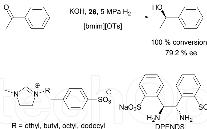
Fig. 31. Hydrogenation of acetophenone using tosylate imidazolium ILs and DPENDS
