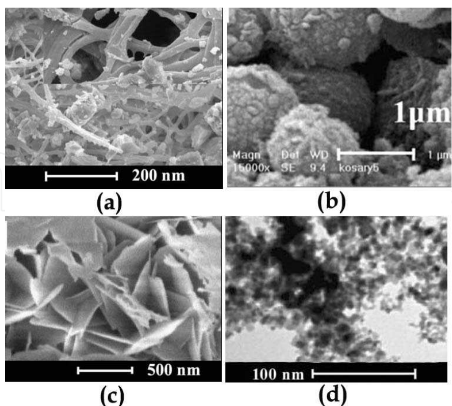
Fig. 9. SEM images of PANI/ \text{Y}_2\text{O}_3 composite at different type of IL: (a) PANI/ \text{Y}_2\text{O}_3 composite ( \text{Y}_2\text{O}_3 = 30\% , aniline = 0.2 M, and IL = [\text{hepmim}]^+\cdot\text{H}_2\text{PO}_4^- = 0.6 \text{ M} ), (b) PANI/ \text{Y}_2\text{O}_3 composite ( \text{Y}_2\text{O}_3 = 30\% , aniline = 0.2 M, and IL = [\text{hepmim}]^+\cdot\text{HSO}_4^- = 0.6 \text{ M} ), (c) PANI/ \text{Y}_2\text{O}_3 composite ( \text{Y}_2\text{O}_3 = 30\% , aniline = 0.2 M, and IL = [\text{hepmim}]^+\cdot\text{NO}_3^- = 0.6 \text{ M} ). (d) TEM image of \text{Y}_2\text{O}_3 (Reproduced from Kowsari & Faraghi (2010) Ultrason. Sonochem. 17, 4, 718-725, Copyright (2010), with permeation from Elsevier)
