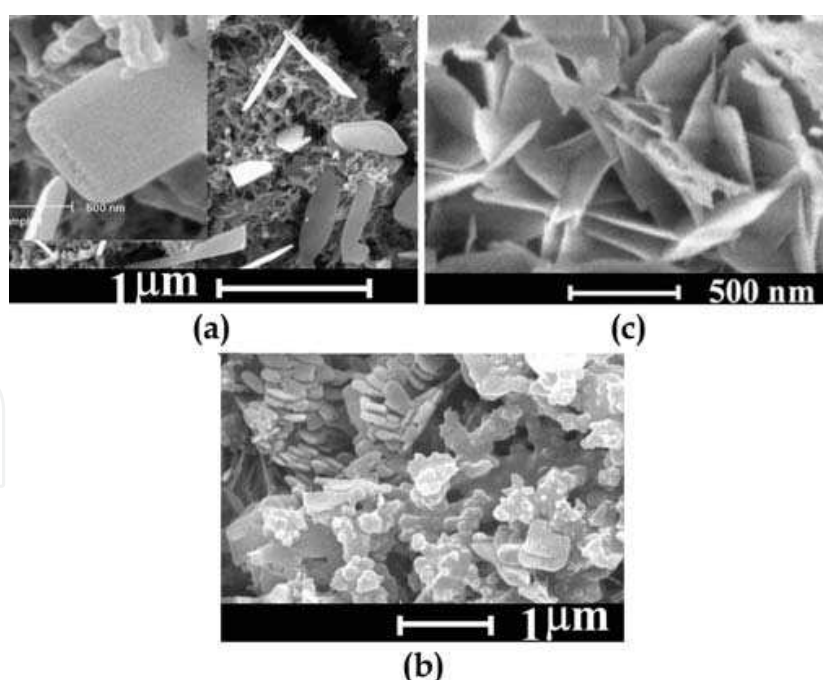
Fig. 11. SEM images of PANI/ \text{Y}_2\text{O}_3 composite ( \text{Y}_2\text{O}_3 = 30\% , aniline = 0.2 M, and IL = [hepmim] \text{HSO}_4 ) at different concentrations of ILs (a) [IL] = 0.2 M, (b) [IL] = 0.4 M, (c) [IL] = 0.6 M (Reproduced from Kowsari & Faraghi (2010) Ultrason. Sonochem. 17, 4, 718-725, Copyright (2010), with permission from Elsevier)
