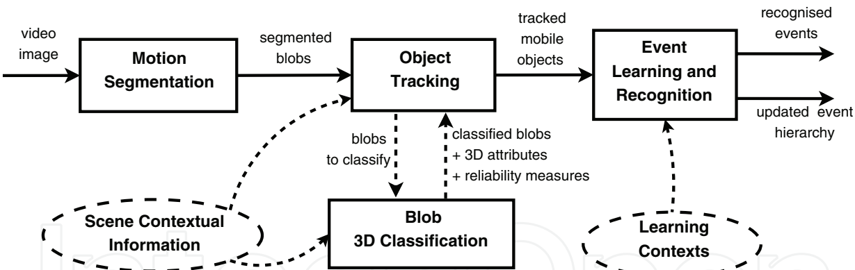
Fig. 1. Proposed video understanding approach.
