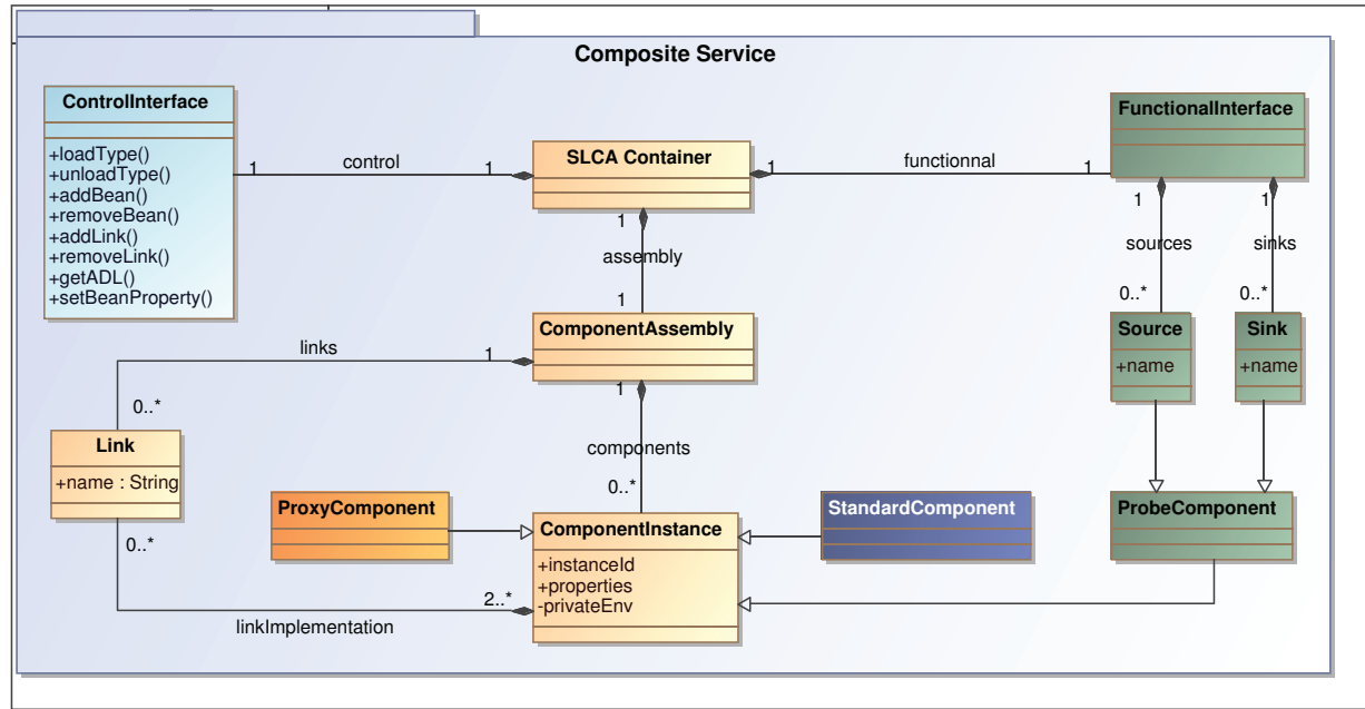
Fig. 9. SLCA Metamodel : composite services interfaces
