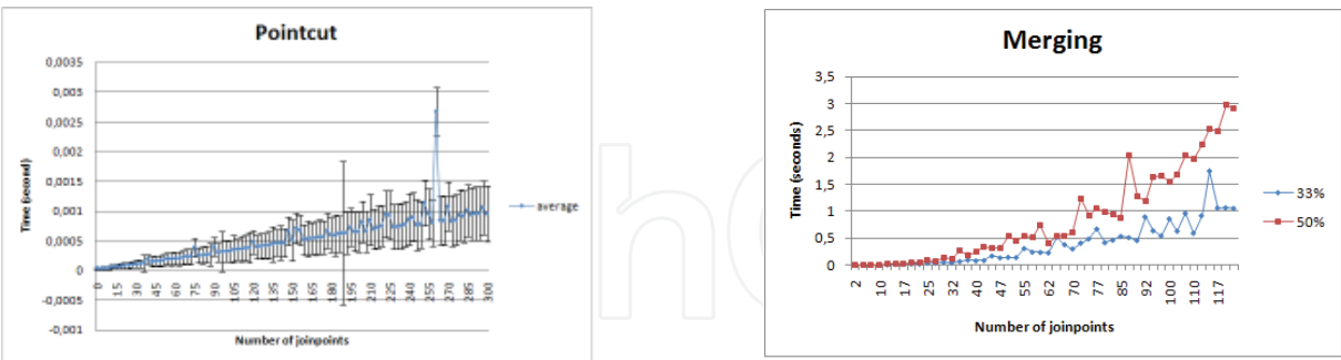
Fig. 20. Pointcut matching and merging time measures.
