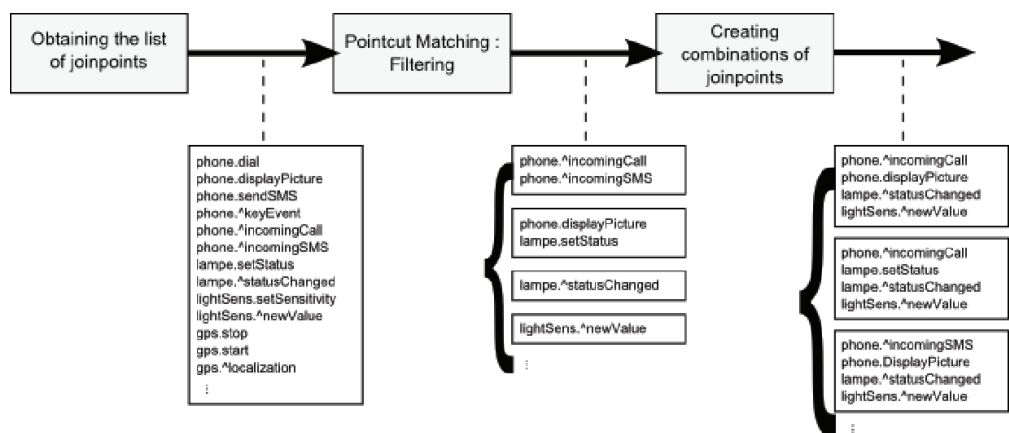
Fig. 12. Example of pointcut matching process
