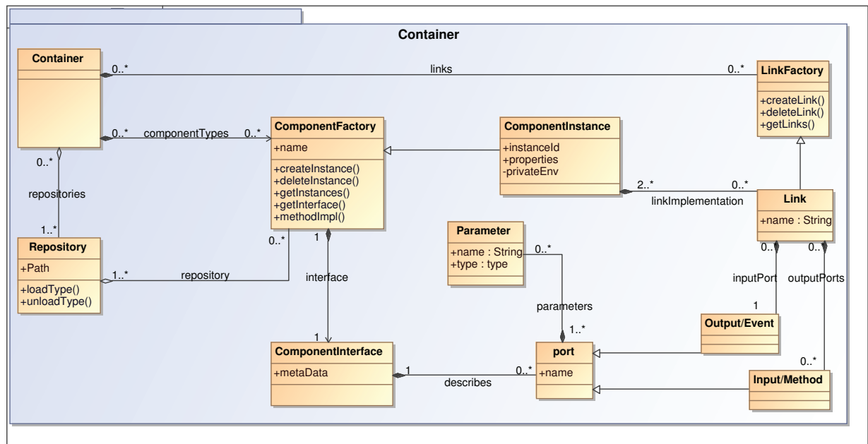
Fig. 6. LCA meta-model: lightweight components
