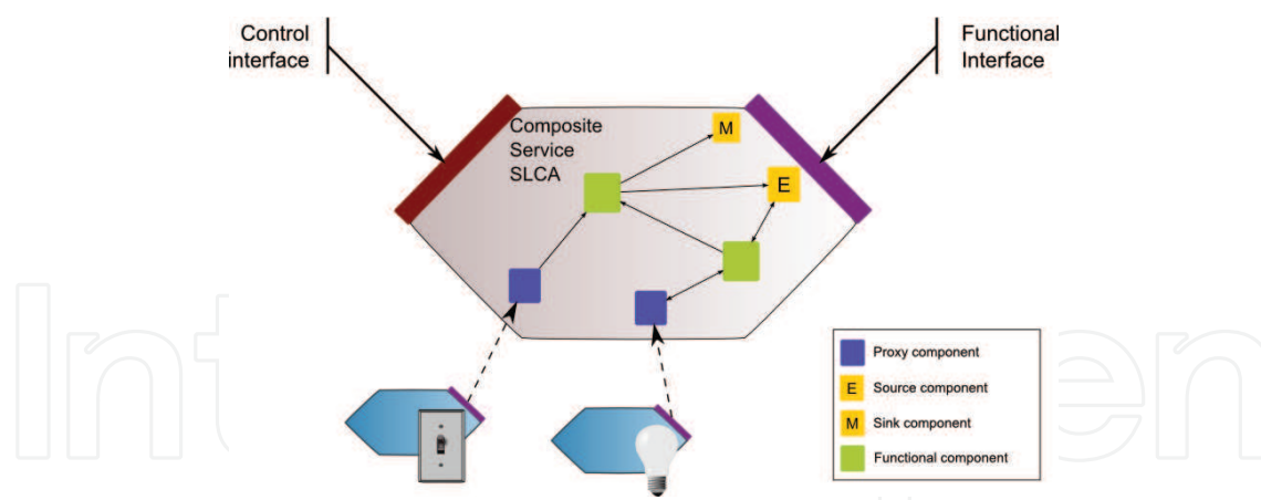
Fig. 7. Composite web service with evented communications
