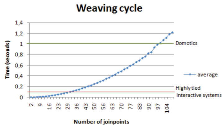
Fig. 21. Weaving time measures.
