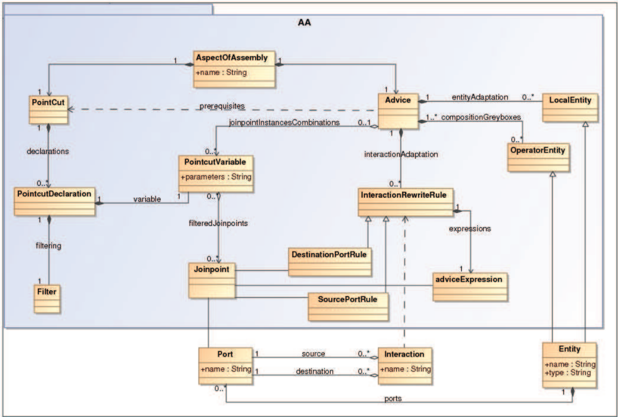
Fig. 11. Aspect of Assembly meta-model
