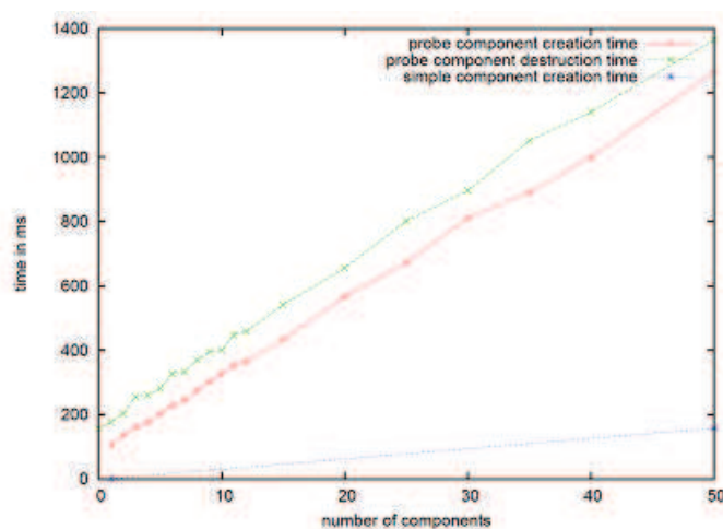
Fig. 19. Component creation and destruction time measures.
