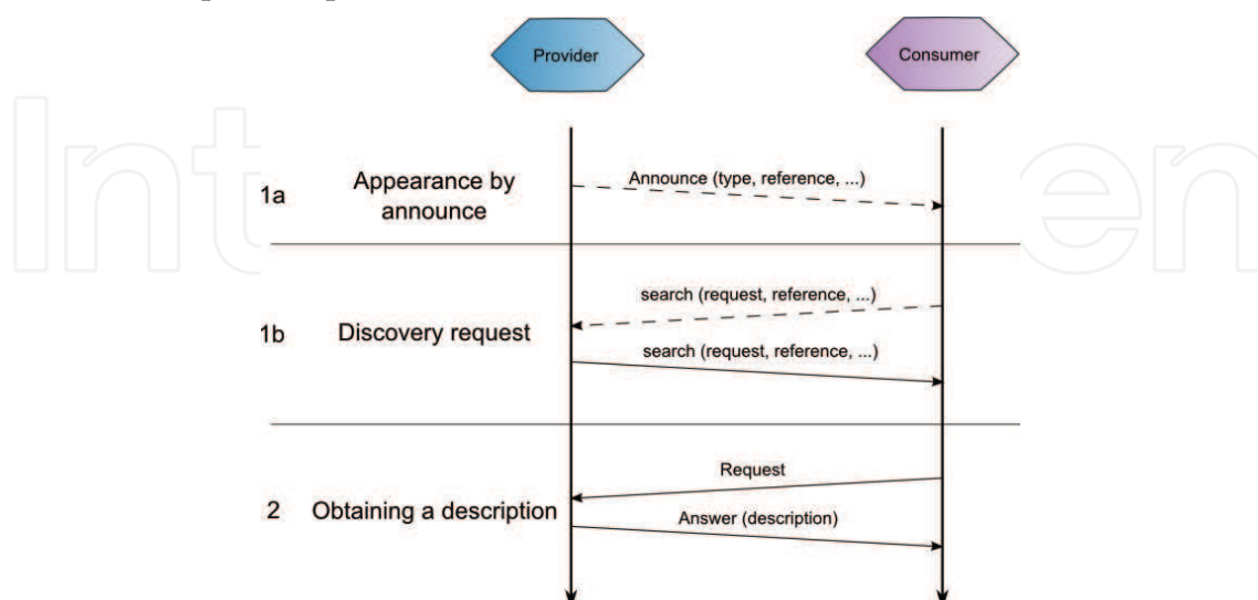
Fig. 4. Dynamic decentralized discovery : discovery and search protocols
