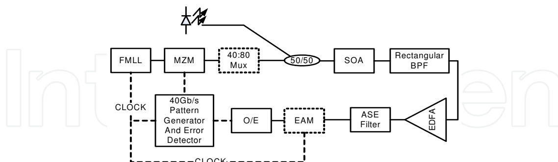
Fig. 6. Experimental set-up
