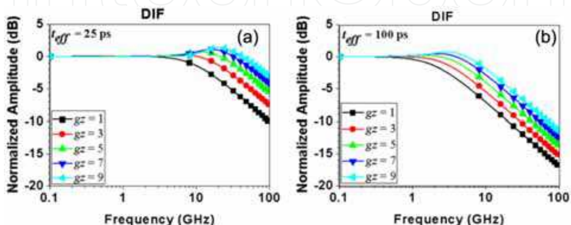
Fig. 7. Normalized frequency response for the differentially biased SOA-MZI AOWC, (a) for t_{eff} 25 ps (b) for t_{eff} 100 ps
