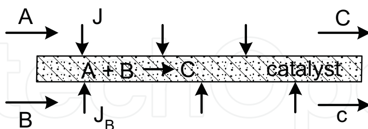
Fig. 1. Schematic illustration of catalytic membrane reactor
