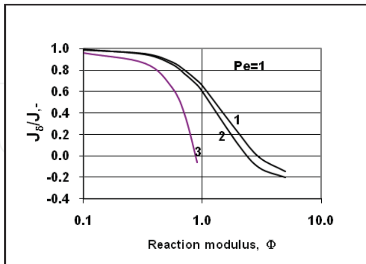
Fig. 11. The relative value of outlet mass transfer rate as a function of reaction modulus applying the Michaelis-Menten kinetics (line 2) and its limiting cases, namely first-order (line 1) and zero-order kinetics. ( D_m=5.4 \times 10^{-10} \text{ m}^2/\text{s} ; C_\delta^0 = 0 ; \beta^0 = \beta_\delta^0 \rightarrow \infty ; K_M/c^0=1 ; \delta_m=100 \text{ }\mu\text{m} )
