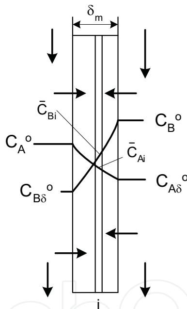
Fig. 3. Illustration of the concentrations for second-order reaction
