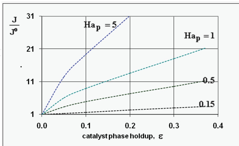
Fig. 4. The mass transfer rate as a function of the catalyst phase holdup obtained by the pseudo-homogeneous model ( H_m=H=1 ; D_m=1 \times 10^{-10} \text{ m}^2/\text{s} ; C_\delta^0 = 0 ; \beta^0 = \beta_\delta^0 \rightarrow \infty ; d_p=2 \text{ }\mu\text{m} ; \delta_m=30 \text{ }\mu\text{m} )
