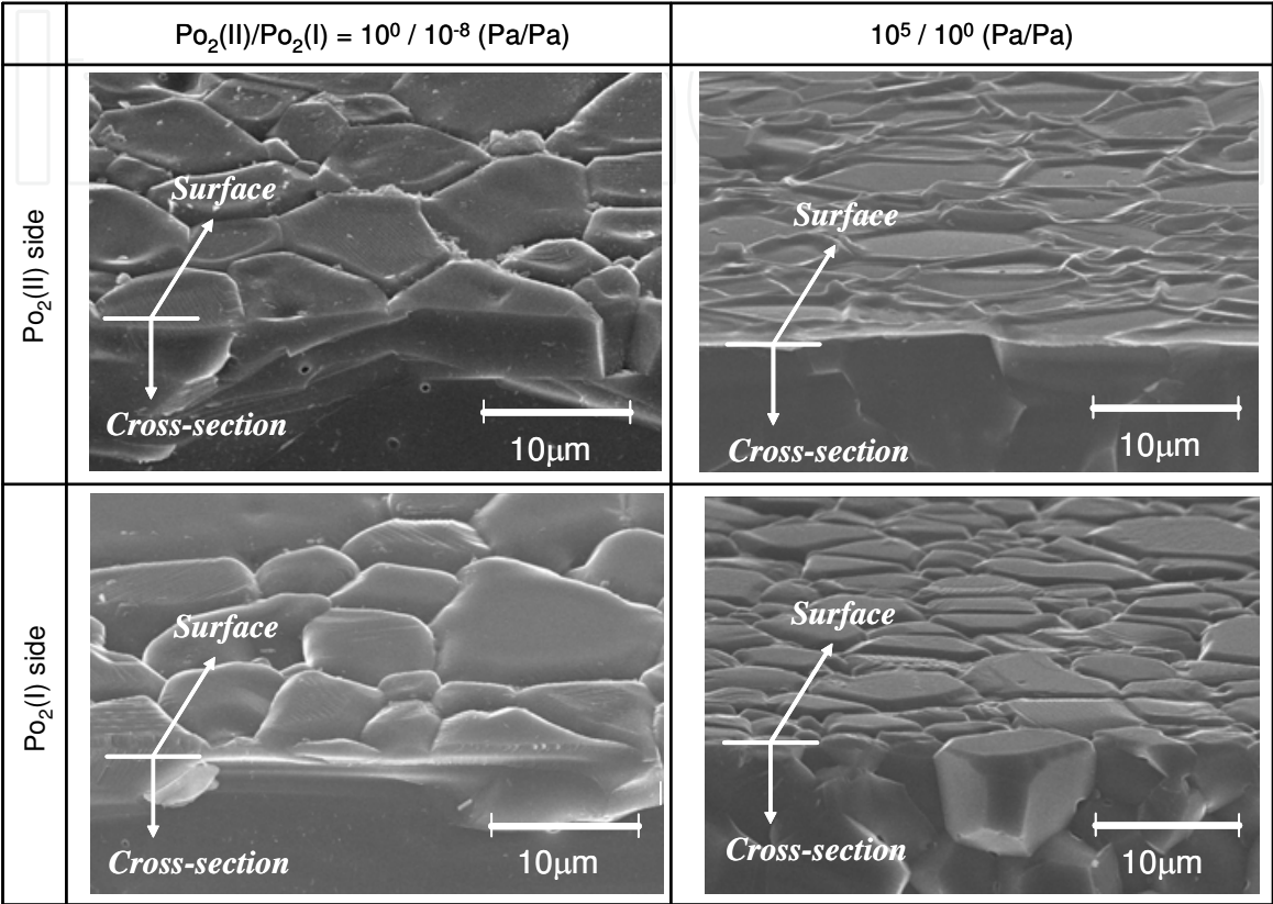
Fig. 10. shows SEM micrographs of the surfaces and cross-sections of non-doped polycrystalline alumina exposed at 1923K for 10h under \Delta P_{O_2} with P_{O_2}(II)/P_{O_2}(I)=1 Pa/ 10^{-8} Pa and 10^5 Pa/1 Pa.
