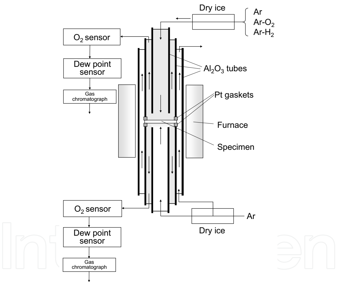
Fig. 7. Schematic diagram of the gas permeability apparatus.
