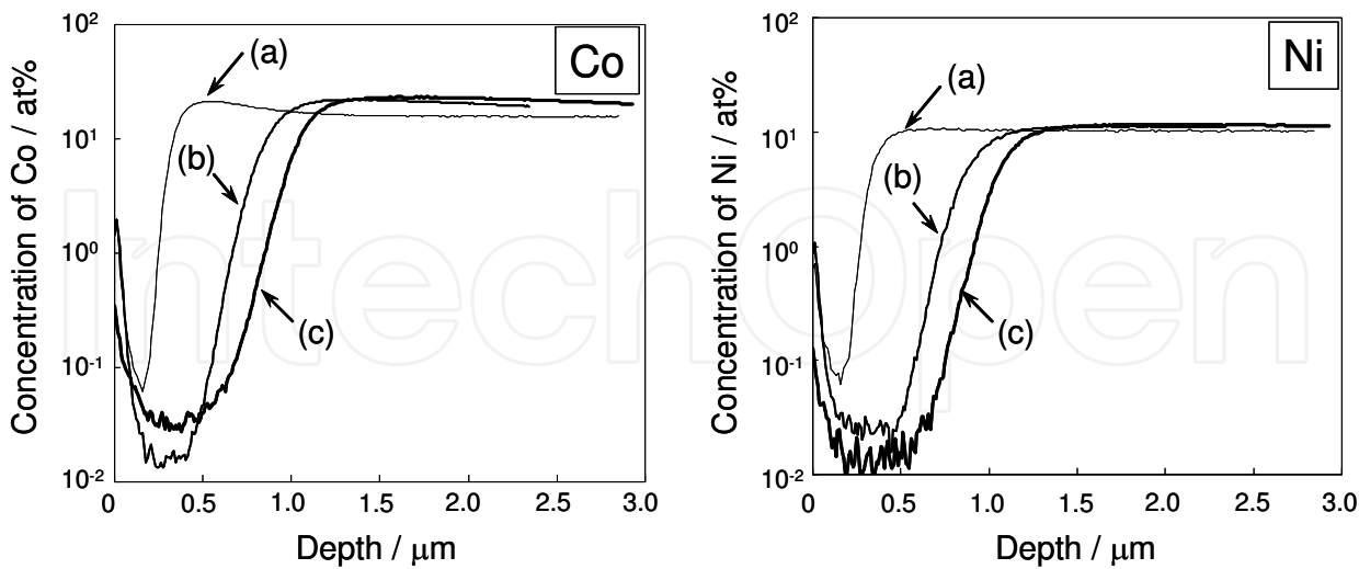
Fig. 6. SIMS depth profiles of Co and Ni through the CoNiCrAlY coats of the samples oxidized at a holding temperature of 1323 K under a \text{P}_{\text{O}_2} of 10^{-14} Pa. Lines (a) and (b) in Fig. 8 are when the temperature was increased to 1323 K according to \text{P}_{\text{O}_2} along line A in Fig.5 and then held for 10 and 600 min, respectively. Line (c) in Fig. 6 is when the temperature was increased to 1323 K according to \text{P}_{\text{O}_2} along line B in Fig. 5 and then held for 600 min.
