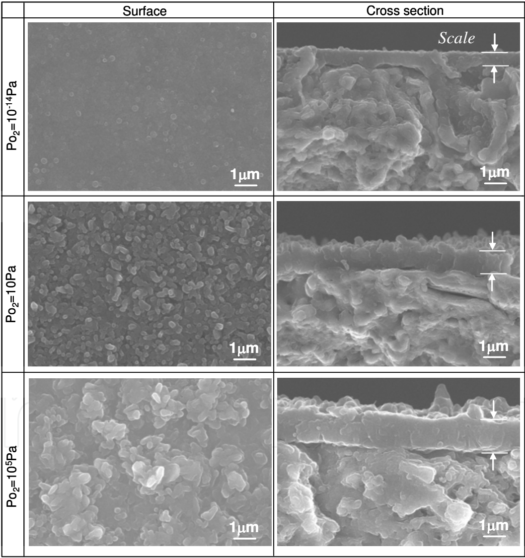
Fig. 3. SEM micrographs of the surfaces and cross-sections of the samples oxidized at 1323 K for 600 min under P O2 of 10 -14 , 10, and 10 5 Pa.
