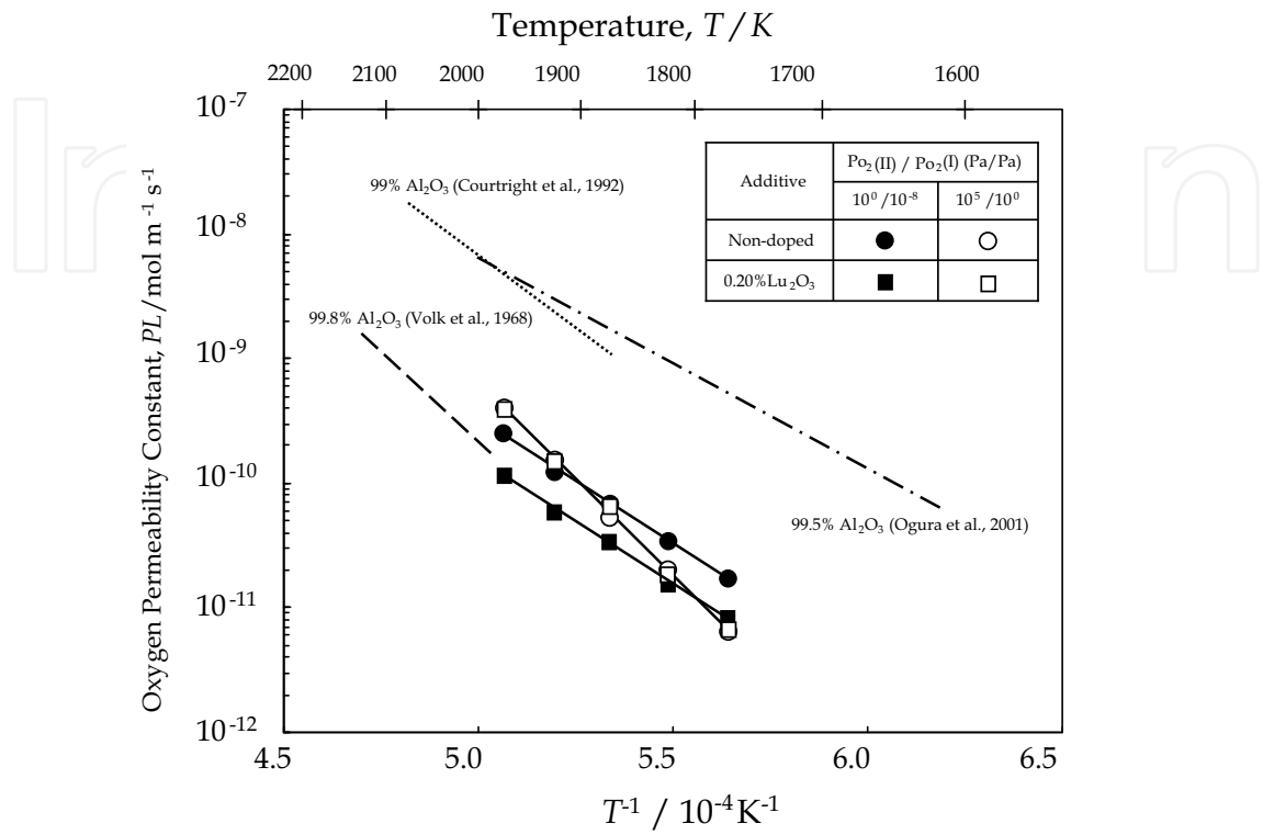
Fig. 8. Temperature dependence of oxygen permeability constant of polycrystalline Al 2 O 3 (non-doped and doped with 0.2 mol% Lu 2 O 3 ) exposed to oxygen potential gradients ( \Delta P_{O_2} ). The solid and open symbols indicate data for specimens exposed under P_{O_2(II)} / P_{O_2(I)} = 1 \text{ Pa} / 10^{-8} \text{ Pa} and 10^5 \text{ Pa} / 1 \text{ Pa} , respectively. The other lines are data from the literature under a similar \Delta P_{O_2} as that for the open symbols.
