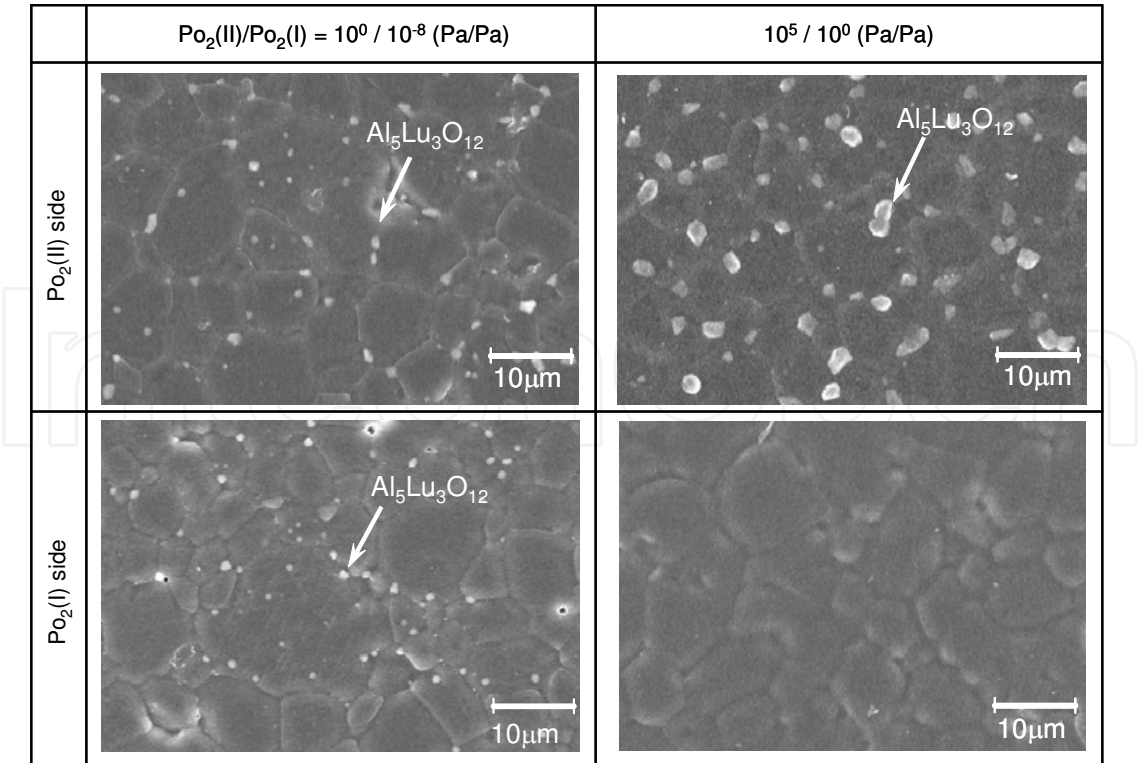
Fig. 12. SEM micrographs of the surfaces of polycrystalline alumina doped with 0.2 mol% \text{Lu}_2\text{O}_3 exposed at 1923K for 10h under \Delta P_{O_2} with P_{O_2(II)}/P_{O_2(I)}=1 \text{ Pa}/10^{-8}\text{Pa} and 10^5\text{Pa}/1\text{Pa} .
