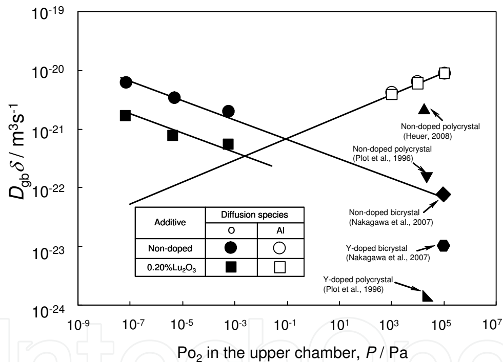
Fig. 13. D_{gb}\delta of oxygen and aluminum in polycrystalline alumina (non-doped and doped with 0.2 mol% \text{Lu}_2\text{O}_3 ) as a function of the equilibrium partial pressures of oxygen in the upper chamber at 1923 K. The solid and open symbols indicate the D_{gb}\delta of oxygen and aluminum, respectively.
