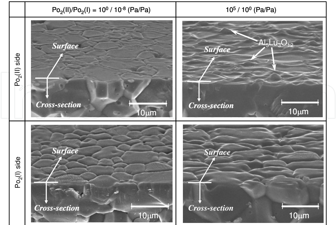
Fig. 11. SEM micrographs of the surfaces and cross-sections of polycrystalline alumina doped with 0.2 mol% \text{Lu}_2\text{O}_3 exposed at 1923 K for 10 h under \Delta P_{O_2} with P_{O_2(II)}/P_{O_2(I)}=1 \text{ Pa}/10^{-8} \text{ Pa} and 10^5 \text{ Pa}/1 \text{ Pa} .
