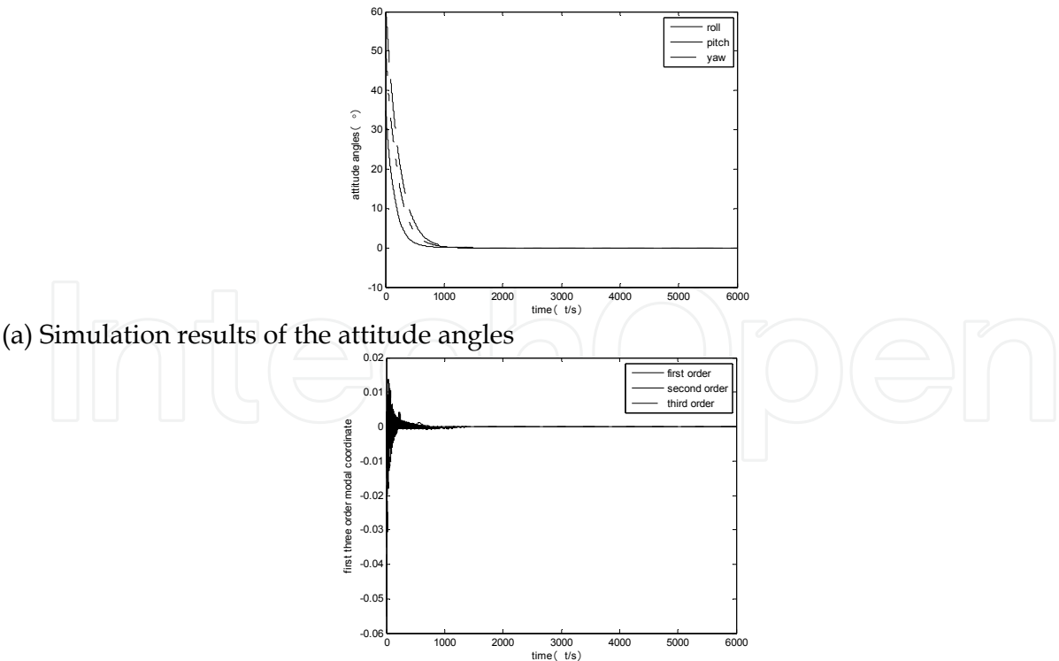
(b) Simulation results of the modal coordinates
