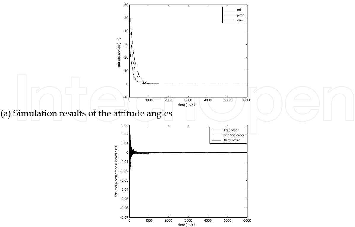
(b) Simulation results of the modal coordinates
