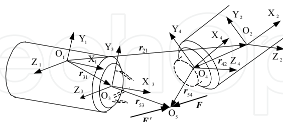
Fig. 29. Action and counteraction between spacecrafts
