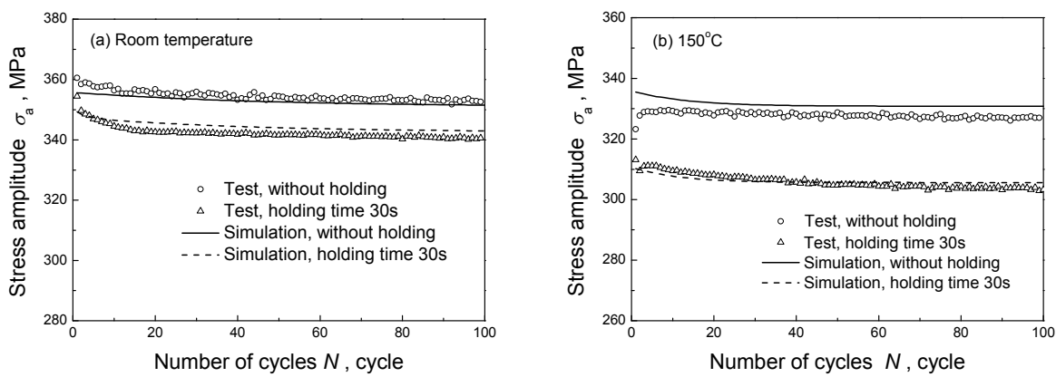
Fig. 13. Experimental and simulated results of responeded stress amplitude vs. number of cycles for 6061-T6 aluminium alloy in the uniaxial symmetrical strain-controlled cyclic loading with strain amplitude of 0.6% and varied hold-time at peak and valley strains: (a) at room temperature; (b) at 150°C. (Originally from Ding et al. (2010))
