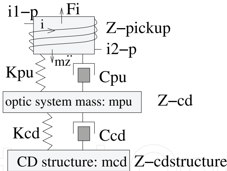
Fig. 10. Mechanical model of the CD structure.
