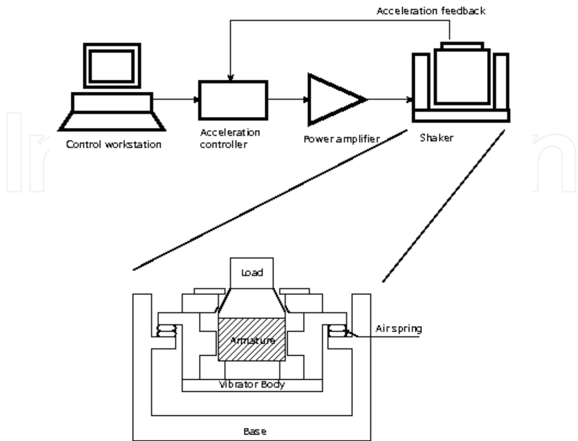
Fig. 4. Block diagram of CD player test configuration.
