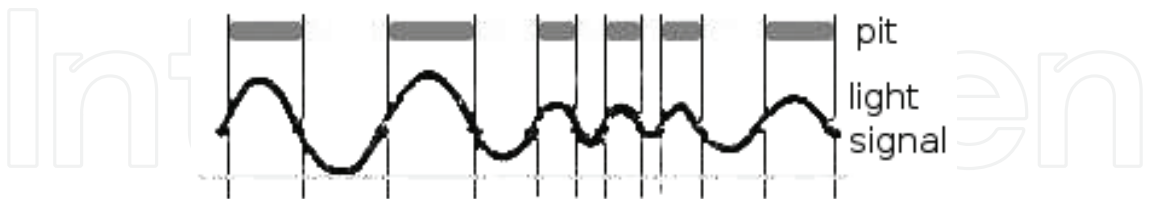
Fig. 12. Example of the EFM modulated light signal received by the photo-diodes when the track reflects back the laser light. Further inputs of this block are position errors generated by the focusing and tracking systems described in section 5.3: in_err_foc and in_err_track . In absence of focusing error, light signals are identical to the sign_foc input. If a focusing error is occurring, light waves are unbalanced towards the correspondent diodes, as described in section 5.4, depending on error sign and on the value of a proper constant K_foc . In the same way the Eee , Eef signals depend on tracking error and the constant K_track . Tolerance factors are defined for both focus and tracking errors.
