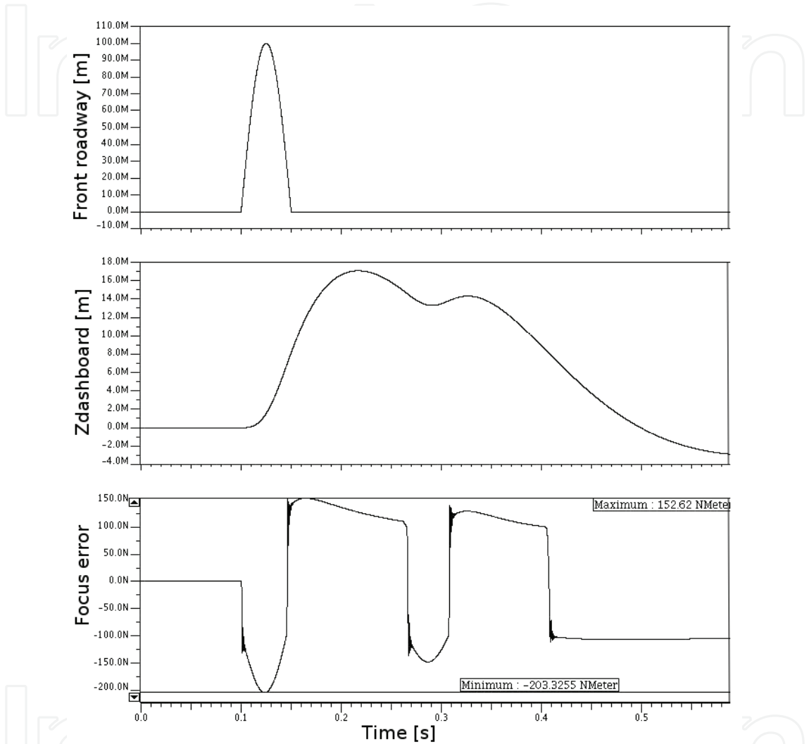
Fig. 14. Dashboard displacement and focus error in case of a bump road profile for a comfort vehicle suspension. No disk radial or vertical shift are used.
