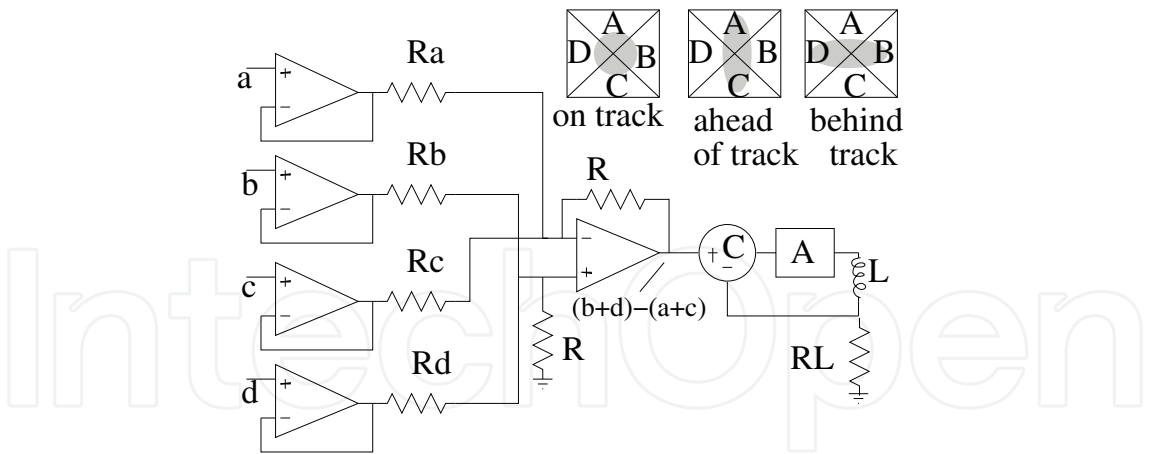
Fig. 11. Focus electrical subsystem.
