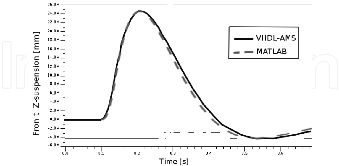
Fig. 9. Suspension displacement ( Z_s ) for a roadway bump profile. Matlab and VHDL-AMS simulation results.
