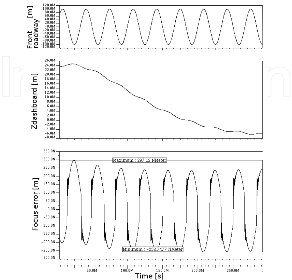
Fig. 15. Dashboard displacement and focus error in case of a sine road profile for a comfort vehicle suspension. No disk radial or vertical shift are used.
