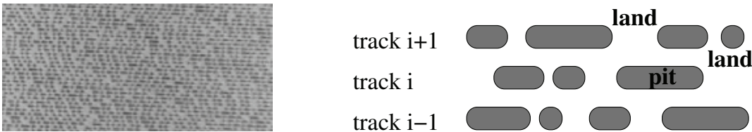
Fig. 2. CD data tracks. Left: photograph (Mansuripur, 1994). Right: detail of three tracks organized in pits and lands.
