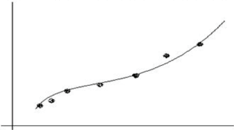
Fig. 10. Logistic regression.
