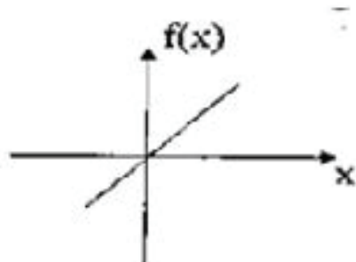
Fig. 3. Identity (Linear) Function f(x) = x, for all x
