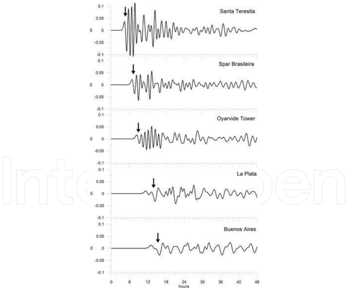
Fig. 6. Simulated sea level oscillation (m) at Santa Teresita, Spar Brasileira, Oyarvide Tower, La Plata and Buenos Aires, forced with wave amplitude equal to 0.03 m at the eastern boundary. Arrows point out the beginning of the activity
