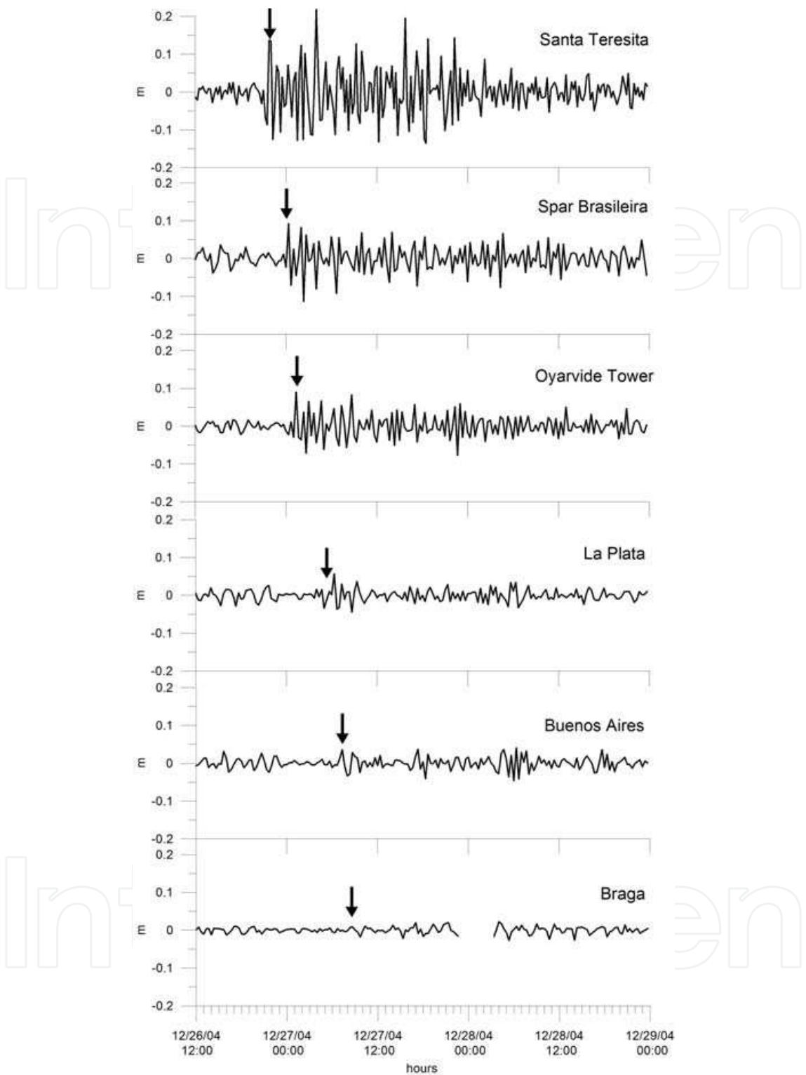
Fig. 4. Passband filtered sea level records (m) at Santa Teresita, Spar Brasileira, Oyarvide Tower, La Plata, Buenos Aires and Braga. Time in hours from December 26, 2004, 12:00 (h = +3). Arrows point out the beginning of the activity The wave speed, c , of long ocean waves could be reasonably approximated by (g h)^{1/2} (e.g., Dean & Dalrymple, 1984) where g is the acceleration due to gravity and h the local depth. According to the expression for c and using the corresponding distances and depths, the
