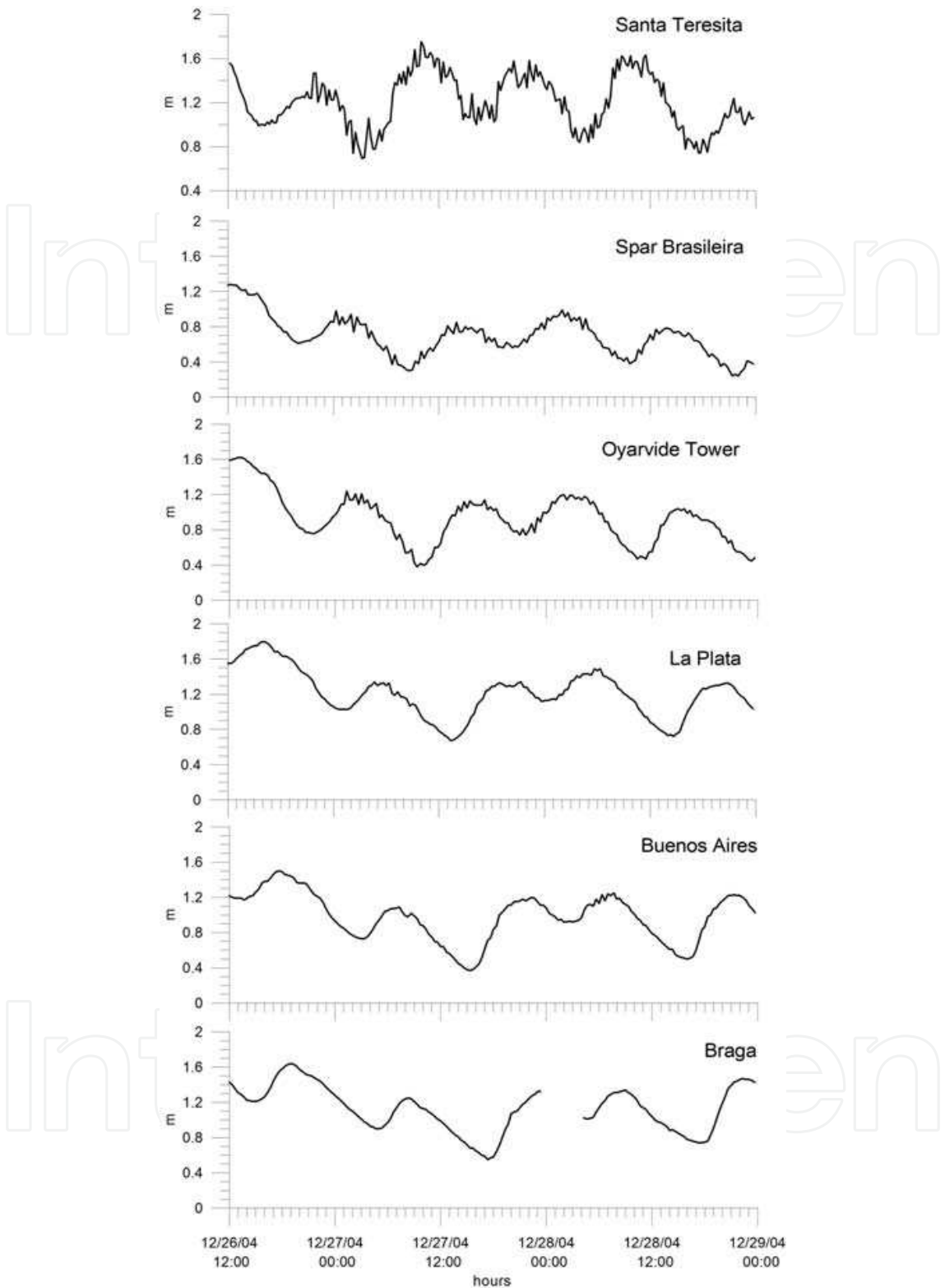
Fig. 3. Sea level records (m) at Santa Teresita, Spar Brasileira, Oyarvide Tower, La Plata, Buenos Aires and Braga. Time in hours from December 26, 2004, 12:00 (h = +3) gauge at Braga did not work between 12/27 23:00 and 12/28 03:00. Sea level data contain diurnal and semidiurnal tides and higher-frequency oscillations ranging from a few minutes to two hours. Water level data were convoluted by means of Kaiser-Bessel bandpass filters
