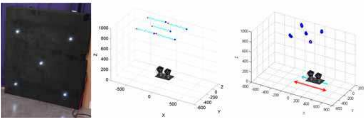
Fig. 17. Landmarks 3D reconstruction with respect to the robot (left) and to the world reference frame (right).
