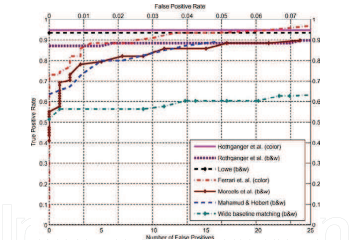
Fig. 11. Performance comparison reported in Rothganger et al. ((2006)).
