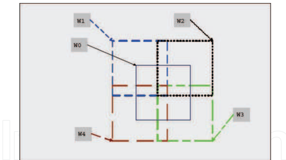
Fig. 6. Multi-window approach for correlation estimation
