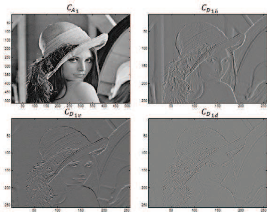
Fig. 3. 1-level discrete wavelet transform of Lena image using figure 2 filter bank
