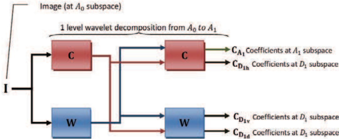
Fig. 2. Mallat’s dyadic wavelet filter bank
