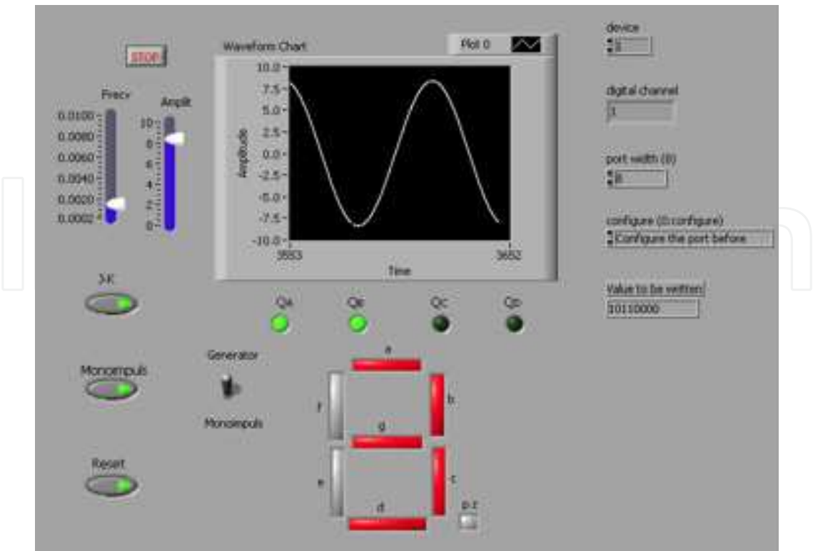
Fig. 13. Front Panel for Controlling the Numeric Display SN7545 thorough Port B(1) of the KPCI-3102 Board
