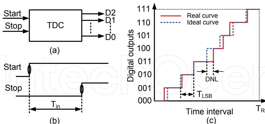
Fig. 1. Basis of time-to-digital conversion.
