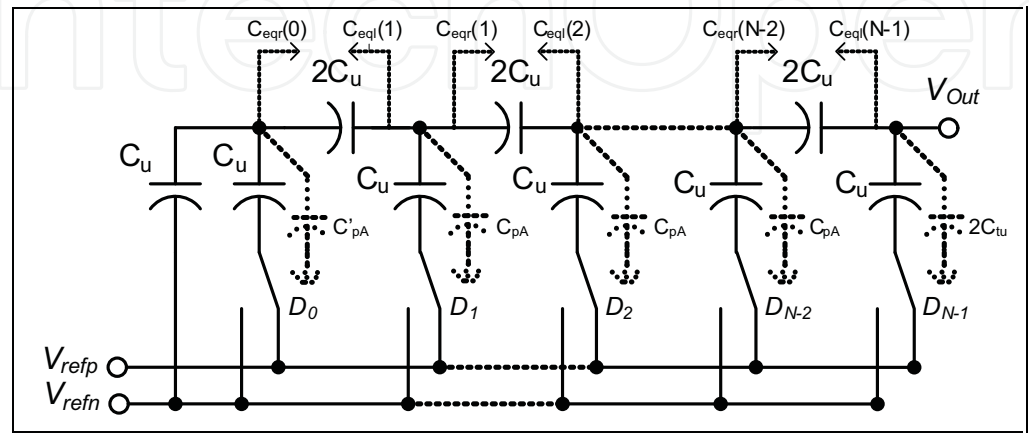
Fig. 4. Parasitic capacitances on C-2C structure
