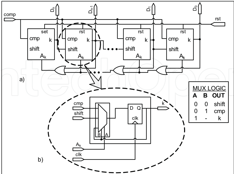
Fig. 13. Schematic of the Successive Approximation Logic The cell is based on the circuit presented in (Oguey and Aebischer, 1997), where the resistor has been replaced by an nMOS transistor working below saturation. The added transistors M2 and M1 provide the gate voltage for M3. The generated current reference I_{ref} is given by:
