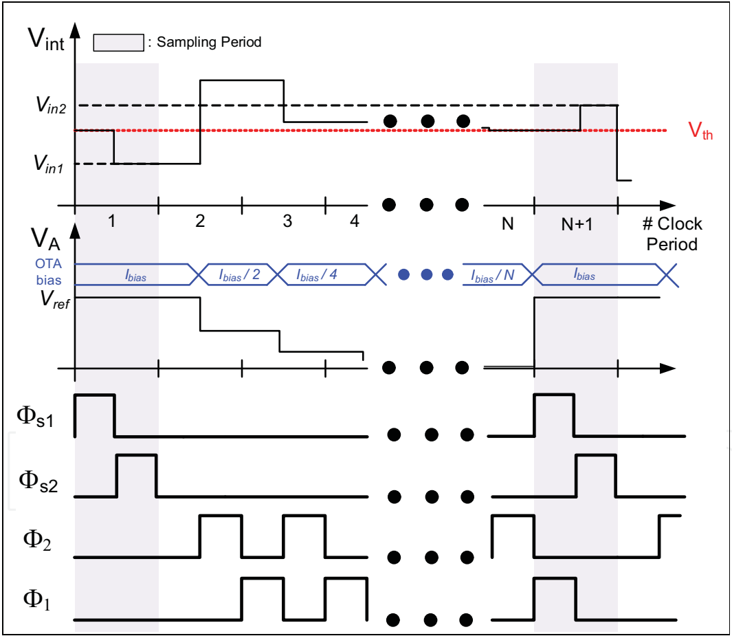
Fig. 7. Waveform of the Binary Search Algorithm implementation
