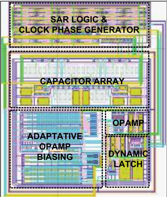
Fig. 19. Layout of the SC-based ADC The layout of the complete ADC is presented in Fig. 19. It occupies an area of 190um x 225um.
