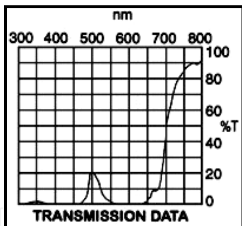
Fig. 15. CDMS – Transmission spectra of used optical filters
