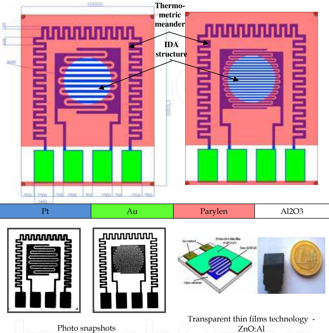
Fig. 1. IDAT microelectrodes
