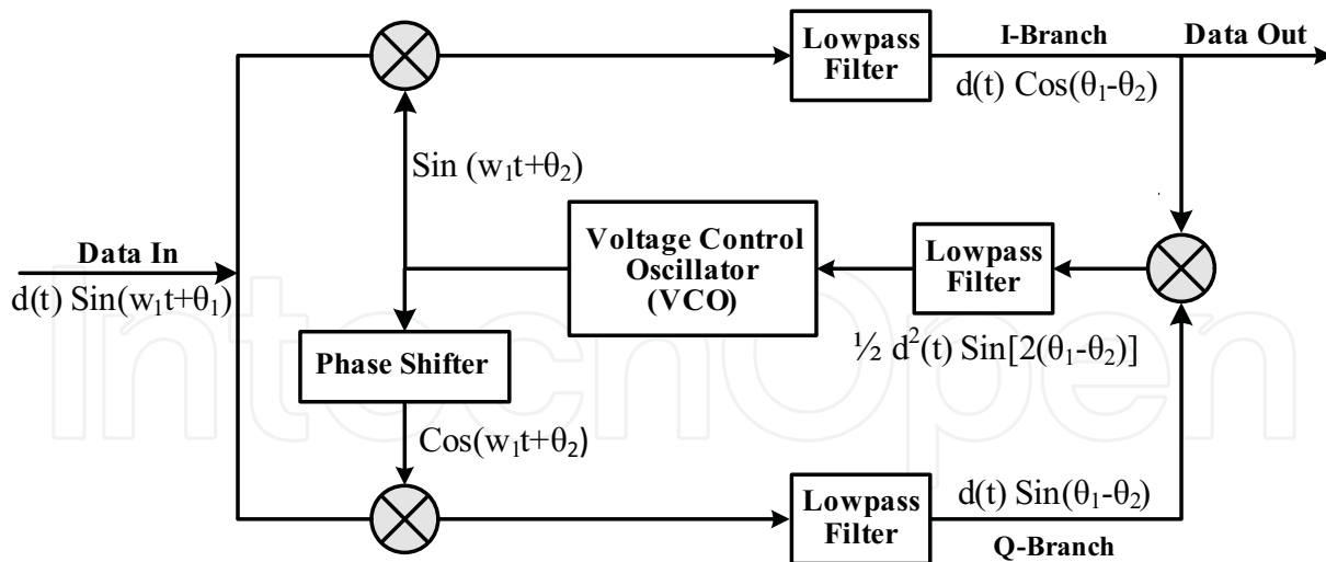
Fig. 15. COSTAS loop for BPSK demodulation.
