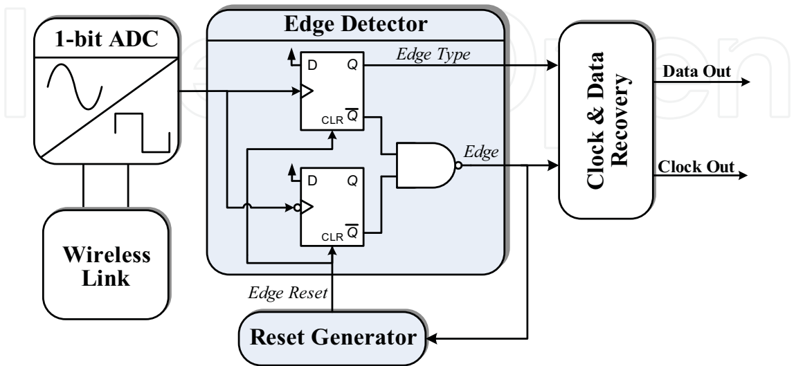
Fig. 16. General block diagram of two noncoherent demodulators presented in (Gong et al., 2008) and (Asgarian & Sodagar, 2009a).
