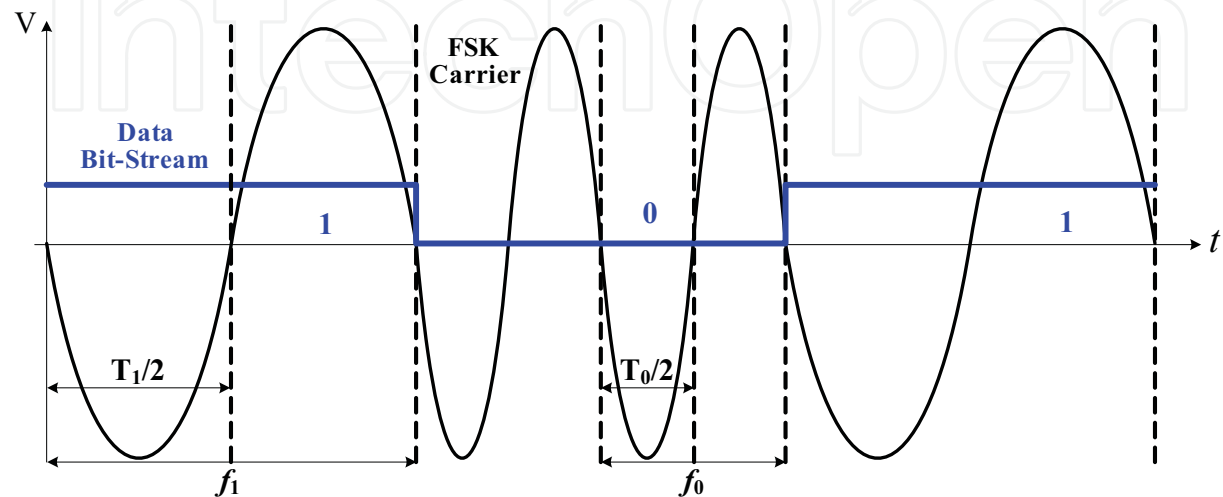
Fig. 13. Phase-coherent BFSK Modulation.
