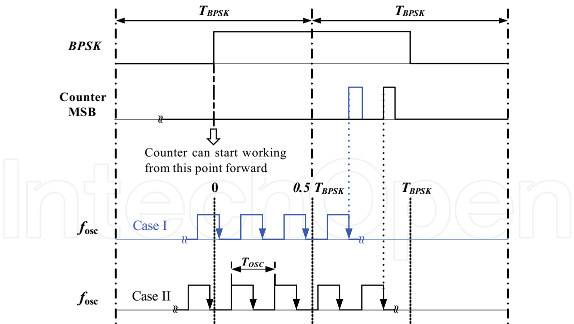
Fig. 17. Two worst cases for determining the range of f_{\text{osc}} in (Asgarian & Sodagar, 2009a) Both of the described noncoherent BPSK demodulators have much lower power consumption than their coherent counterparts. Moreover, they can provide data rates equal to the carrier frequency provided that phase shifts are propagated through the wireless link quickly. In inductive links, this usually requires a low quality factor for the resonant circuits
