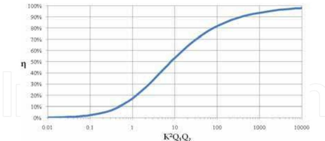
Fig. 4. Maximum achievable link efficiency as a function of K^2 Q_1 Q_2
