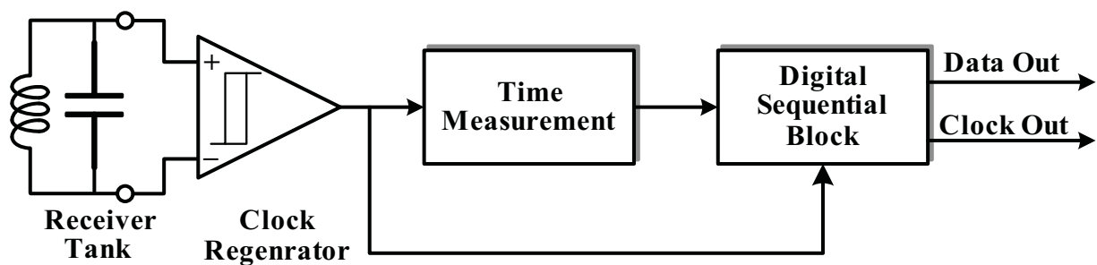
Fig. 14. General block diagram of the demodulators presented in (Ghovanloo & Najfi, 2004)
