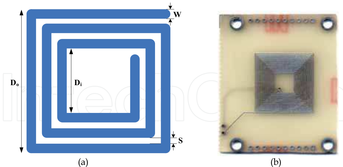
Fig. 6. Typical squared-shaped PSCs. (a) Important geometrical parameters. (b). A prototype fabricated on a printed circuit board (PCB) .
