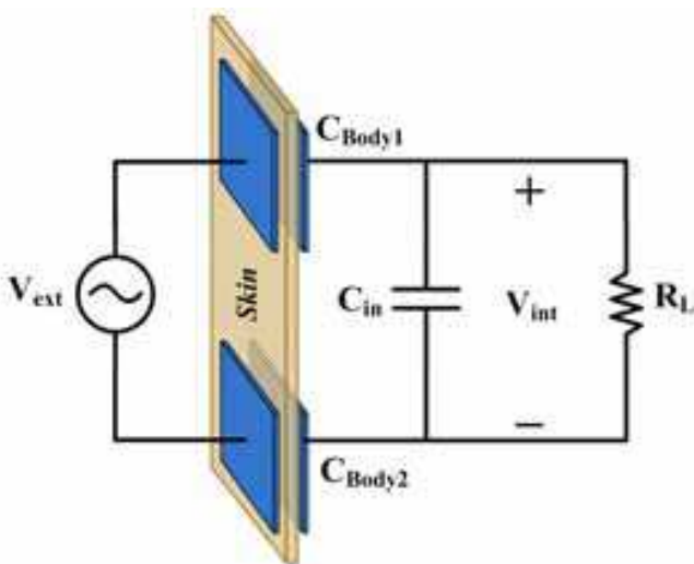
Fig. 8. Simplified schematic of a capacitive link.
