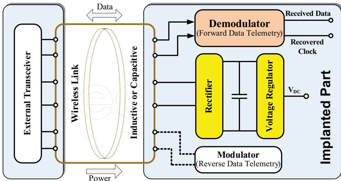
Fig. 1. General block diagram of the wireless interface.
