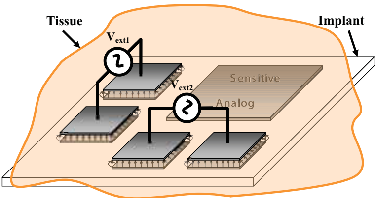
Fig. 7. Energy confinement in the capacitive coupling approach.
