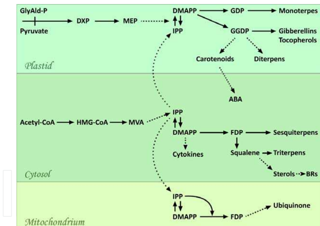
Fig. 9. The pathway of terpenoid biosynthesis
