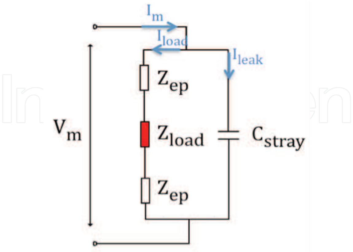
Fig. 2. Electrical equivalent of a EBI measurement setup with a parasitic capacitance in parallel with the impedance load.
