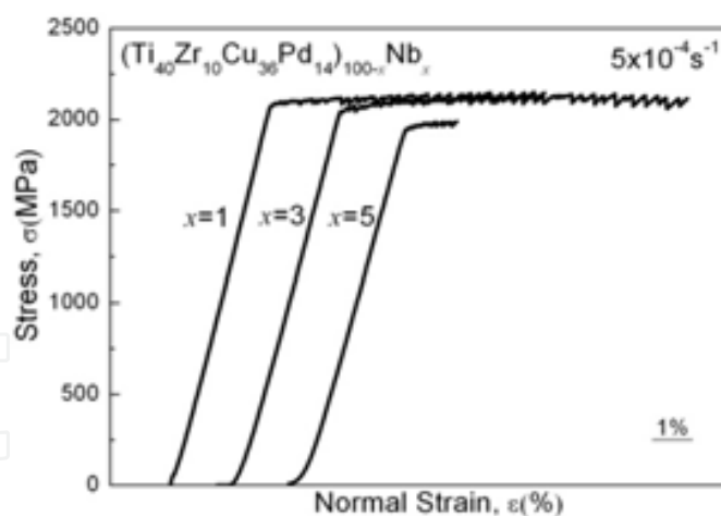
Fig. 7. Compressive strain-stress curves of the (\text{Ti}_{40}\text{Zr}_{10}\text{Cu}_{36}\text{Pd}_{14})_{100-x}\text{Nb}_x as-cast rods with a diameter of 2 mm.
