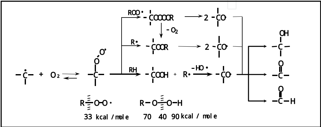
Fig. 3. Peroxy radical formation from carbon-centered radical with molecular oxygen and its reaction, resulted in introduction of oxygen functional groups on polymer surface
