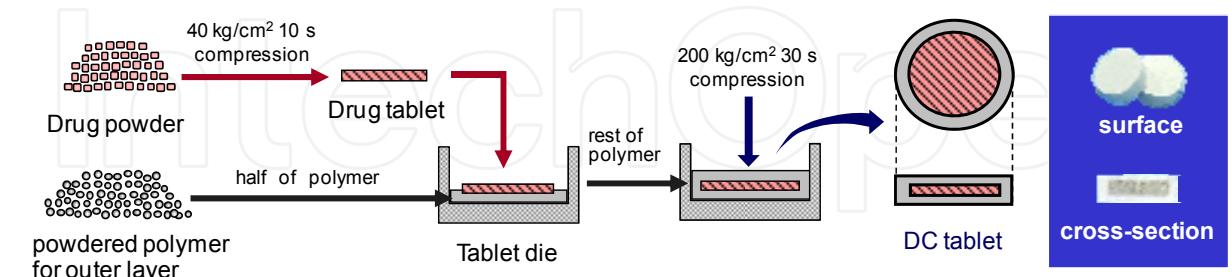
Fig. 7. Schematics for preparation of double-compressed tablets
