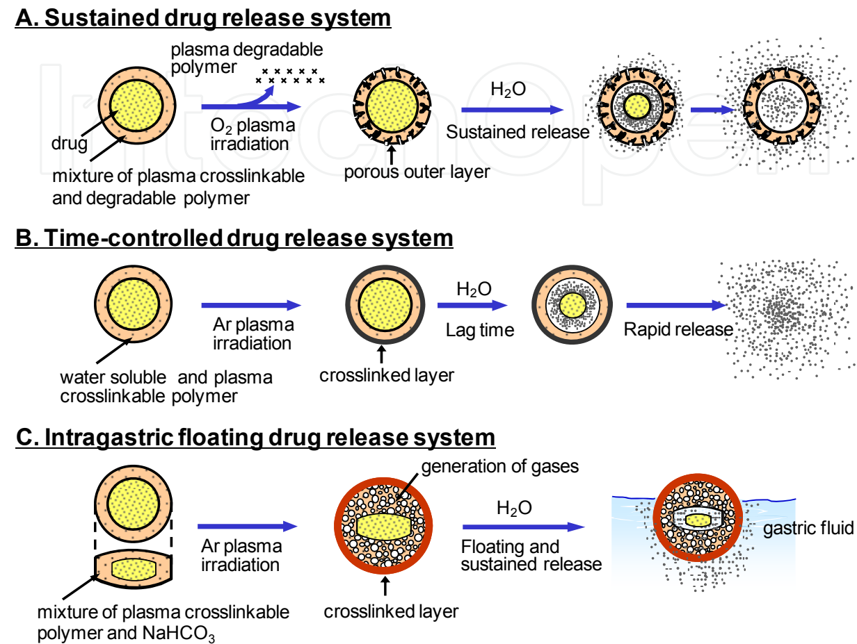
Fig. 6. Conceptual illustration for preparation of DDS for controlled drug release by plasma techniques
