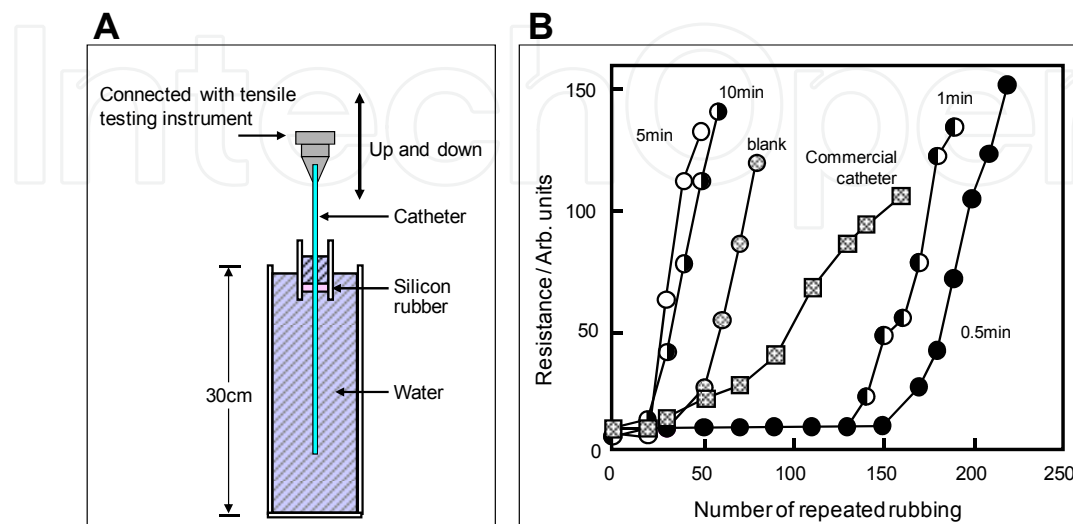
Fig. 24. Experimental setup for measurement of surface lubricity of plasma-irradiated polyurethane-made catheter (A) and durability of the surface lubricity of plasma-assisted VEMAC immobilized catheter in comparison with that of commercial catheter (B)
