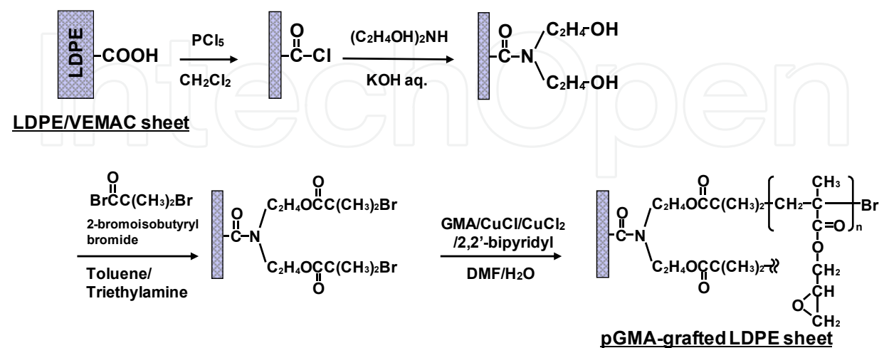
Fig. 27. Reaction scheme for fabrication of pGMA brushes on LDPE sheet by ATRP
