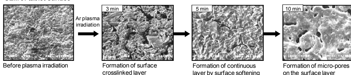
Fig. 14. SEM pictures of Eudragit L100-55 tablet before and after plasma irradiation
