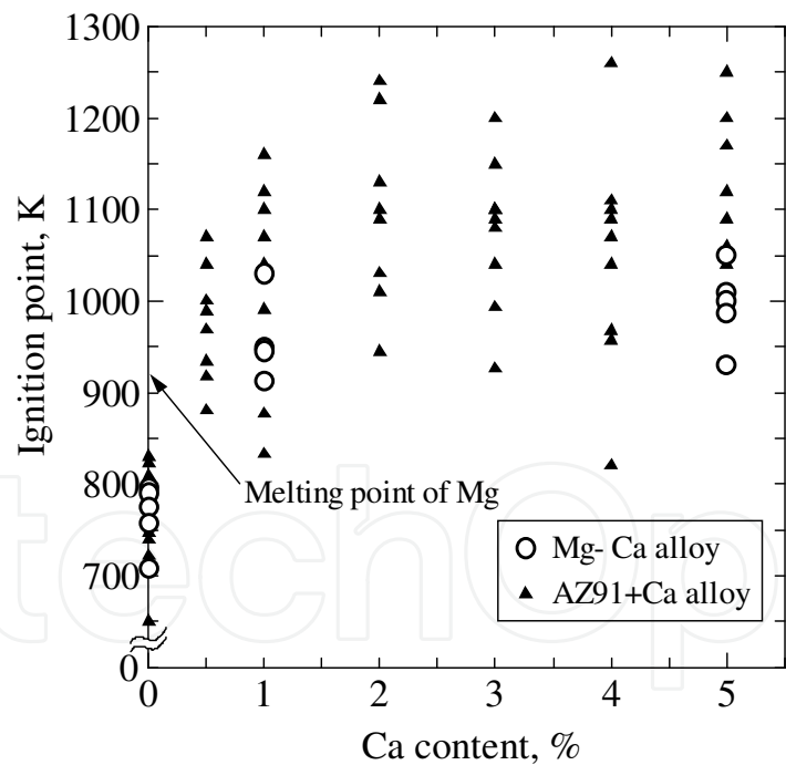
Fig. 3. Relationship between ignition point and Ca content for Mg alloys (Sakamoto et al., 1997)
