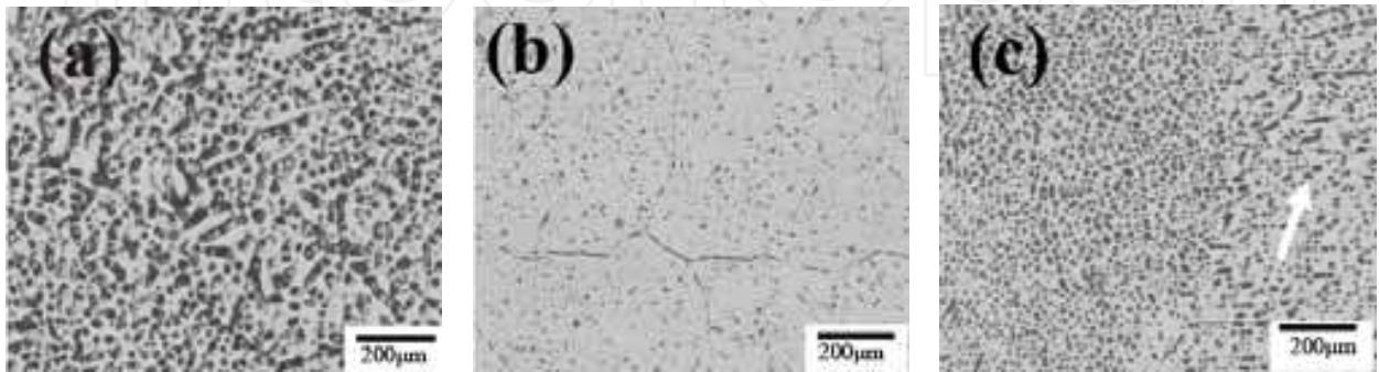
Fig. 3.5. Microstructures of as-cast alloys with different Zn, Y contents: (a) 1#: \text{Zn}/\text{Y}=1/0.23 ; (b) 2#: \text{Zn}/\text{Y}=2/0.46 ; (c) 3#: \text{Zn}/\text{Y}=3/0.69 .
