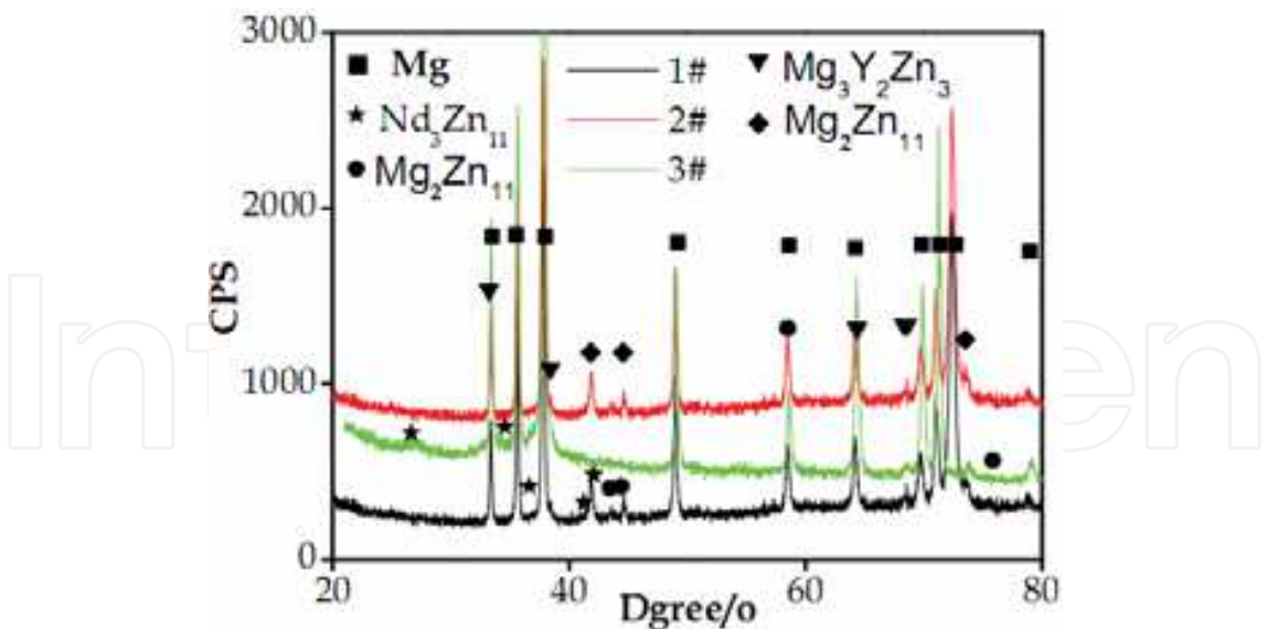
Fig. 3.6 XRD patterns of as-cast alloys (a) 1#alloy (b) 2#alloy (c) 3#alloy
