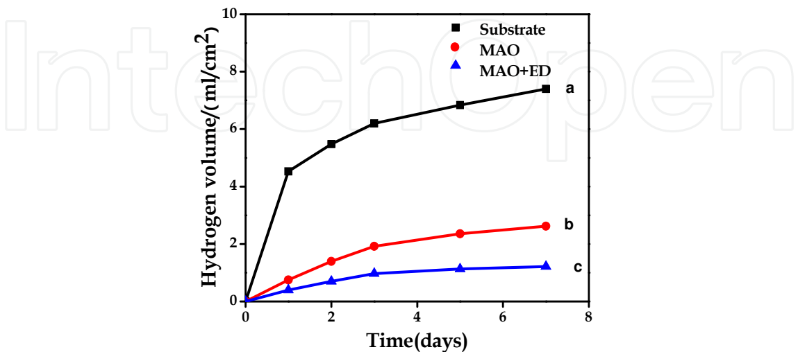
Fig. 4.18. The amount of hydrogen evolution of specimens immersed in SBF: (a) substrate, (b) the MAO/substrate sample and (c) the ED/ MAO/substrate sample.
