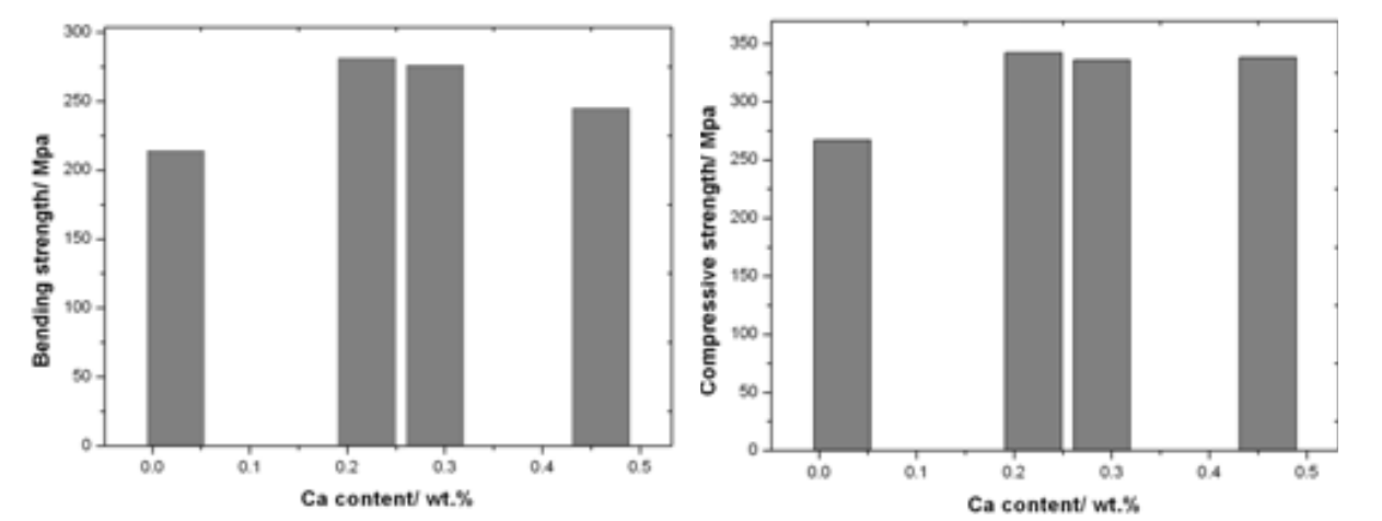
Fig. 3.2. Bending and compression strength of the as-cast alloys with different calcium contents
