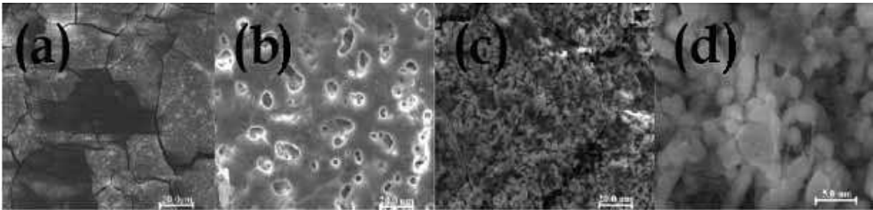
Fig. 4.19. SEM images of corresponding specimens in Fig.4.18 immersed in SBF for 7days ED/ MAO/substrate sample after immersion for 7 days was covered by deposits (Fig.4.19c). The new deposits layer was shown in detail in Fig.4.19 (d), which showed the new layer was composed by many rod-like precipitates. The main elements of the new layer were Ca, P and O, which revealed that the composite coatings could induce the Ca/P salt deposition and had fine biomimetic mineralization ability. The new layer improved the thickness of the composite coatings and further enhanced the protection effect to the substrate. Additionally, the surface morphology evolution of the ED/ MAO/substrate sample after immersion for 7 days proved that the composite coating had better Ca-P salt induction property than that of pure HA coating (Wen, et al, 2009). Fig.4.20 showed the compressive load of the substrate and the ED/ MAO/substrate immersed in SBF for different time. The results of the compressive load and compressive strength of the samples were shown in Tab.5.5 (The corrosion area changed of the cross-section was neglected to calculate the compressive strength). In Fig.4.20, the compressive load and strength of the ED/ MAO/substrate were higher than those of the substrate after 2 and 6 weeks immersion. The results indicated that the composite coatings delayed the strength loss of the Mg-Zn-Ca alloy. As shown in Tab.5.5, the compressive loads of the substrate were decreased to 19.5 KN and 13.9 KN after 2 and 6 weeks immersion, and the compressive strength were 248.2 MPa and 177.2 MPa respectively. Because of the protection of the composite coatings, the compressive load and strength of the ED/ MAO/substrate were 21.7 KN and 276.1 MPa after 2 weeks immersion, and 18.2 KN and 231.1 MPa for 6 weeks immersion. Generally, the compressive strengths of human bones were 100~230 MPa in cortical bone and 2~12 MPa in cancellous bone (A. Rakngarma, 2009). Therefore, the composite coatings effectively delayed the decrease in mechanical properties of the Mg-Zn-Ca alloy, and provided adequate support for the pre-healing of fracture bone.
