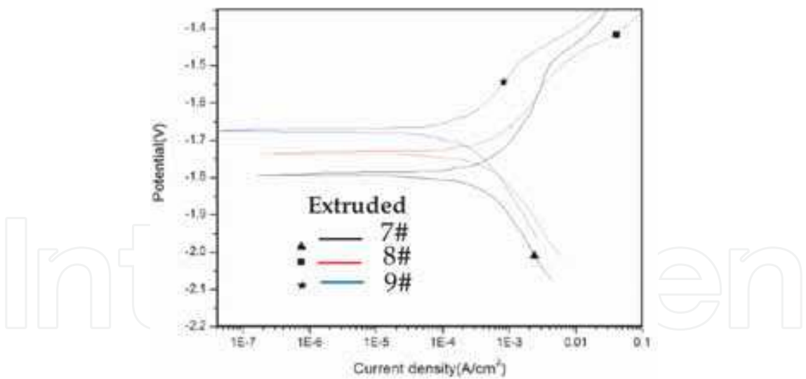
Fig. 3.13. Corrosion polarization curves of the alloys with different Nd content
