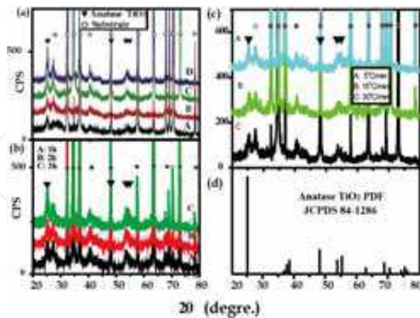
Fig. 4.1. (a) XRD patterns of TiO 2 /AZ31 prepared at the annealing temperature of (A)250 °C,(B)300 °C, (C)350 °C and (D)380 °C for 1.5 h. The diffraction peaks of anatase TiO 2 and AZ31 were shown by the mark of triangle and circle, respectively. (b) XRD patterns of TiO 2 /AZ31 prepared at the annealing temperature of 250 °C for 1h (A), 2h (B) and 3h(C). (c) XRD patterns of TiO 2 /AZ31 prepared at the annealing temperature of 380 °C for 2h with heating rate of 5°C/ min(a), 15°C/ min(b) and 30 °C/ min(c).
