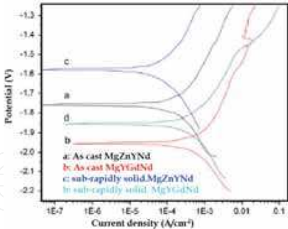
Fig. 3.18. Polarization curves of alloys under different process conditions in dynamic SBF
