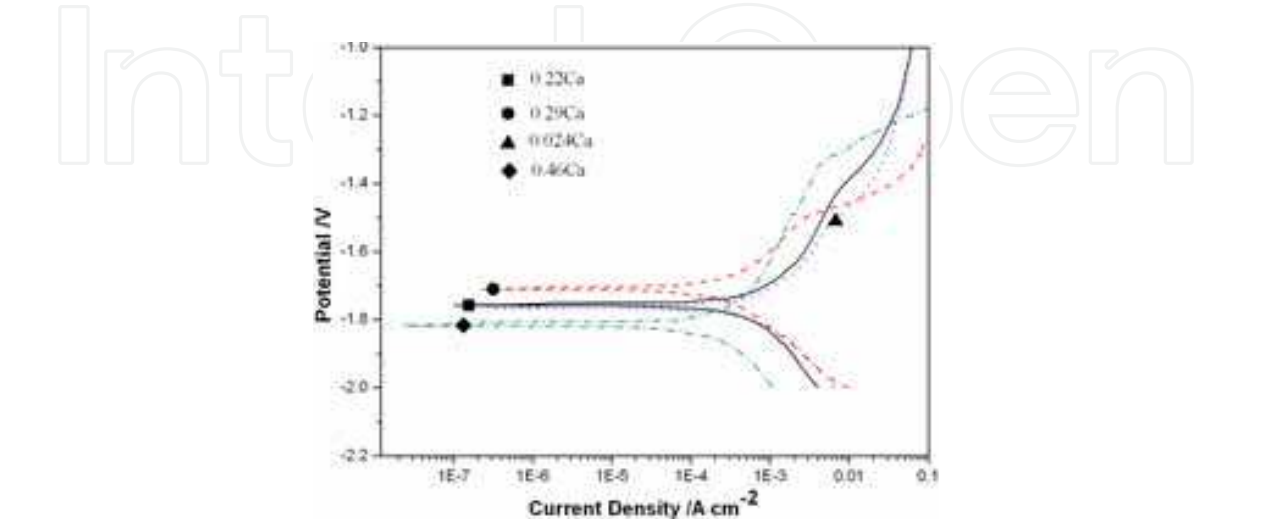
Fig. 3.3. The polarization curves of different alloys in SBF at 37°C
