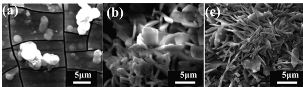
Fig. 4.9. SEM images of corresponding specimens in Fig.4.8 immersed for 7 days.
