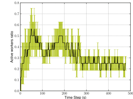
Fig. 9. Self-organized task-allocation
