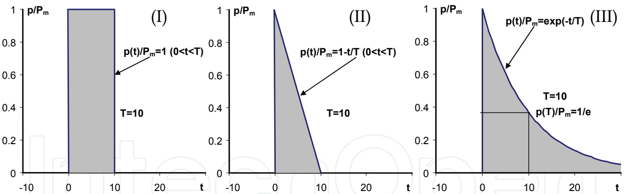
Fig. 7. Typical dynamic pressure functions p(t) used in eq. (16)
