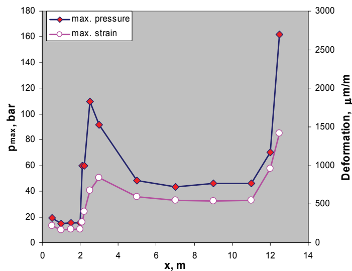
Fig. 15. Maximum pressure load and maximum deformation of the 12.5 m tube under radiolysis gas detonation loads In the case of a later detonation transition ( x_D = 3 m) qualitatively very similar results for calculated pressure load and mechanical response have been obtained. The maximum pipe
