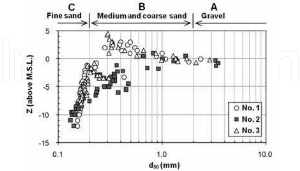
Fig. 12. Depth distribution of d_{50}
