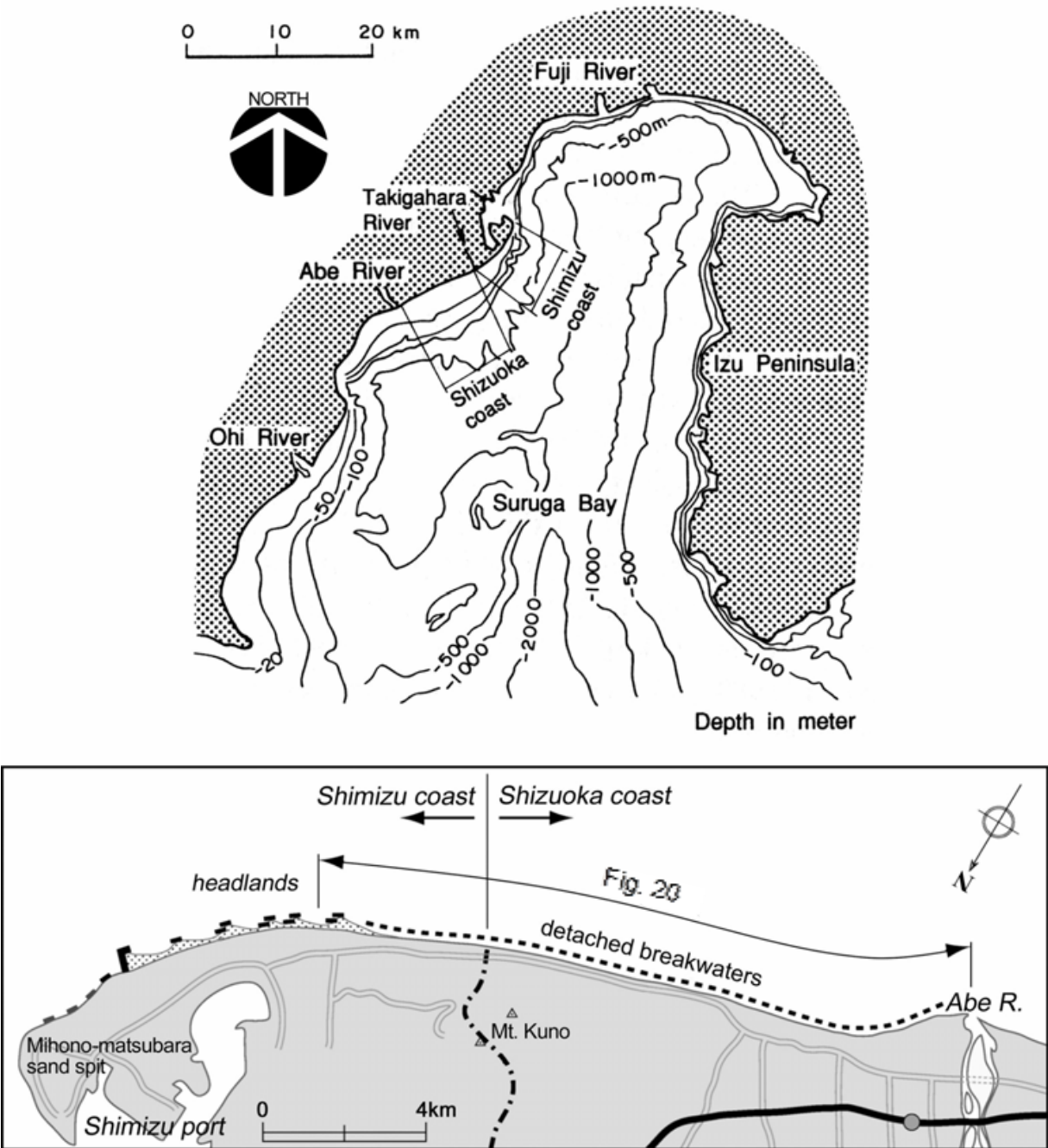
Fig. 19. Location of Shimizu coast
