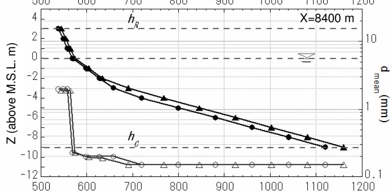
(c) Case 3 Fine materials
