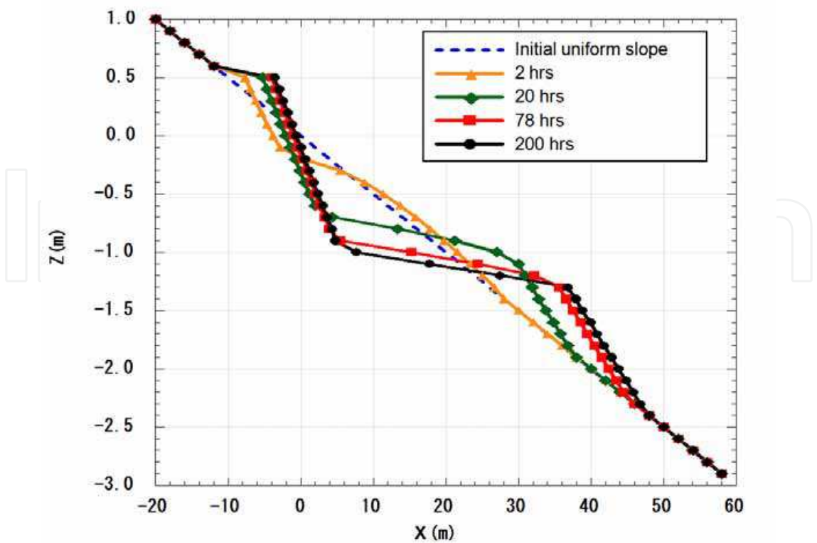
Fig. 5. Change in longitudinal profile with time for contents of fine and coarse sand of \mu^{(1)} =0.7 and \mu^{(2)} =0.3, respectively
