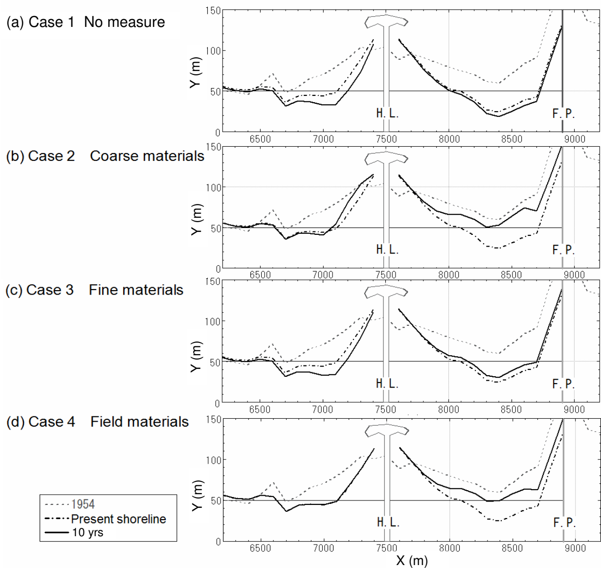
Fig. 17. Shoreline changes in four cases
