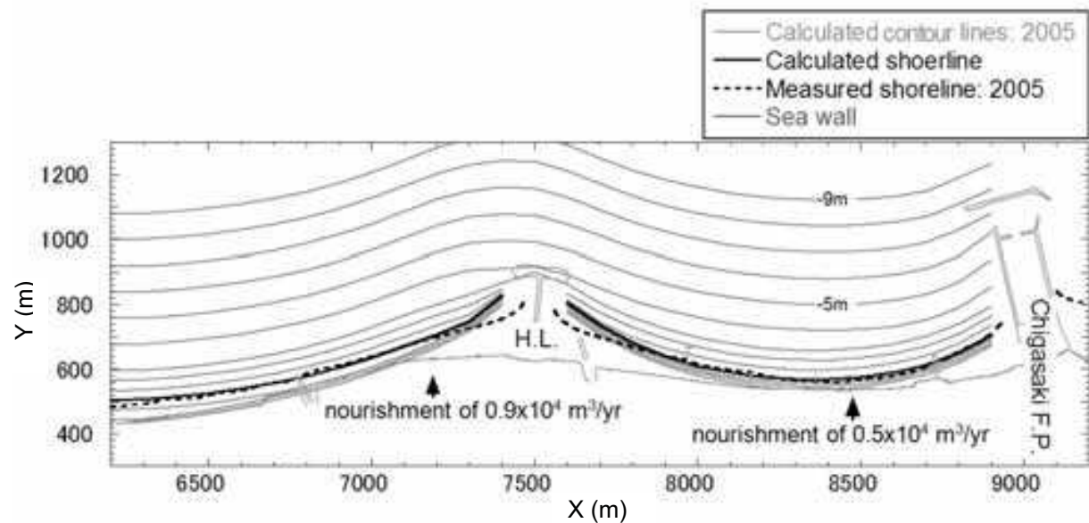
Fig. 14. Reproduced contour lines and comparison of measured and predicted shoreline configurations
