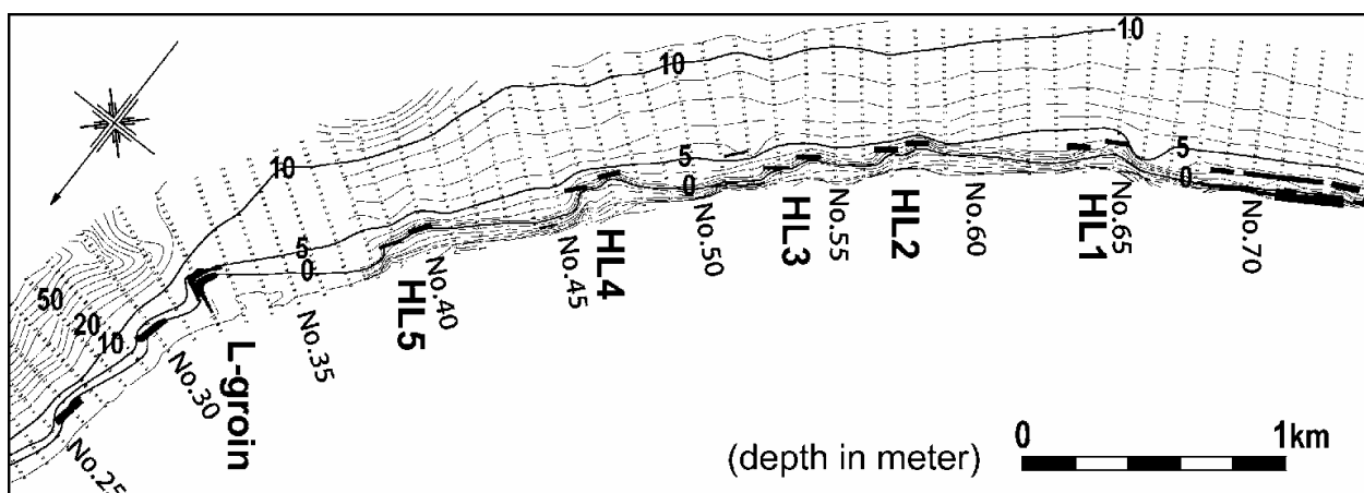
Fig. 20. Bathymetry of Shimizu coast and alignment of transects
