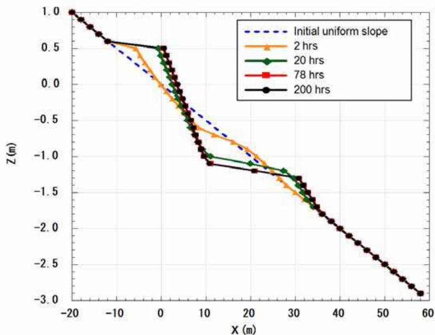
Fig. 9. Predicted changes in longitudinal profile when \mu^{(1)} and \mu^{(2)} are 0.3 and 0.7, respectively
