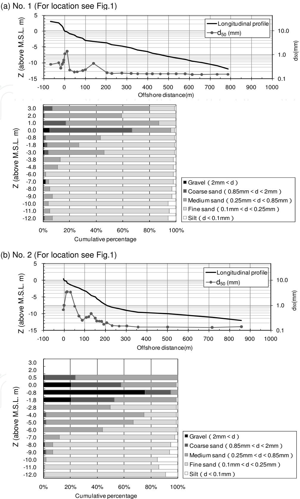
Fig. 13. Longitudinal profiles, cross-shore distributions of d_{50} and contents of grain sizes of bed materials along transect Nos. 1 and 2
