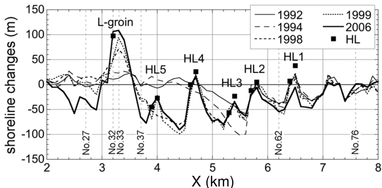
Fig. 21. Shoreline changes with reference to shoreline in 1989
