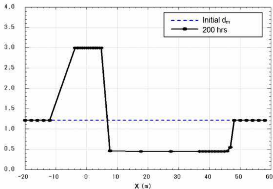
Fig. 8. Cross-shore distribution of mean grain size
