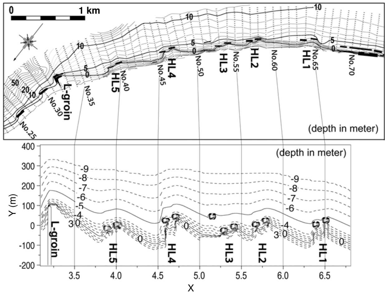
Fig. 24. Calculation domain
