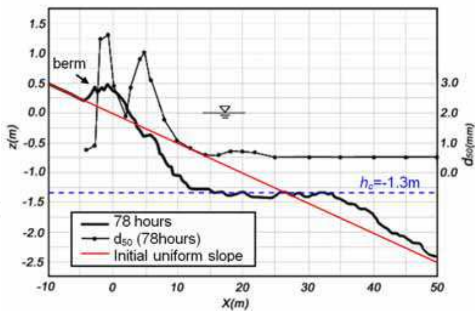
Fig. 3. Change in longitudinal profile and cross-shore distribution of d_{50} in experiment using large wave tank (Meguro et al., 2005)
