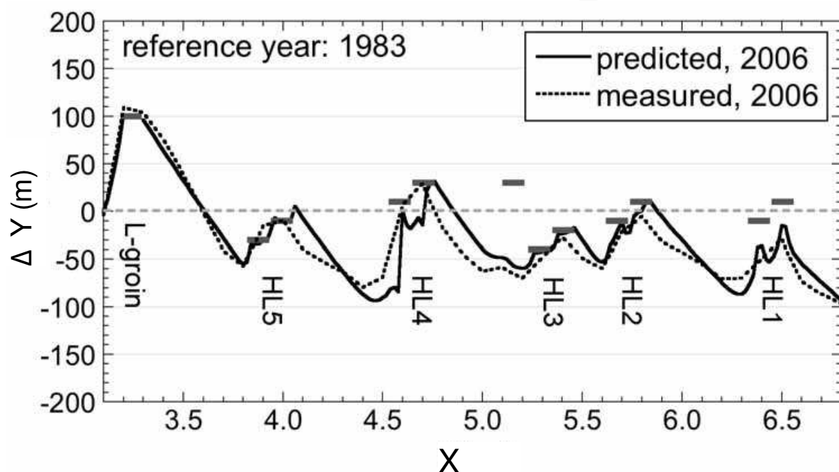
Fig. 26. Measured and predicted shoreline changes
