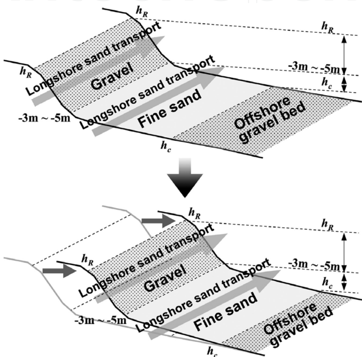
Fig. 23. Schematic explanation of conveyer belts, each carrying mainly gravel and fine sand Along transect No. 27 located north of the L-groin, where the shoreline significantly retreated after the construction of the groin (Fig. 22(f)), the beach slope between the shoreline and a depth of 30 m is as steep as 1/6. Major beach changes are observed up to a
