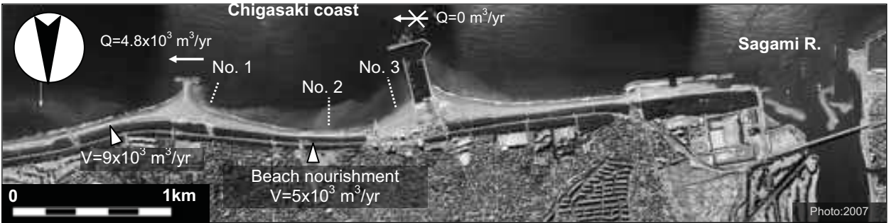
Fig. 11. Aerial photograph of Chigasaki coast and alignment of transects
