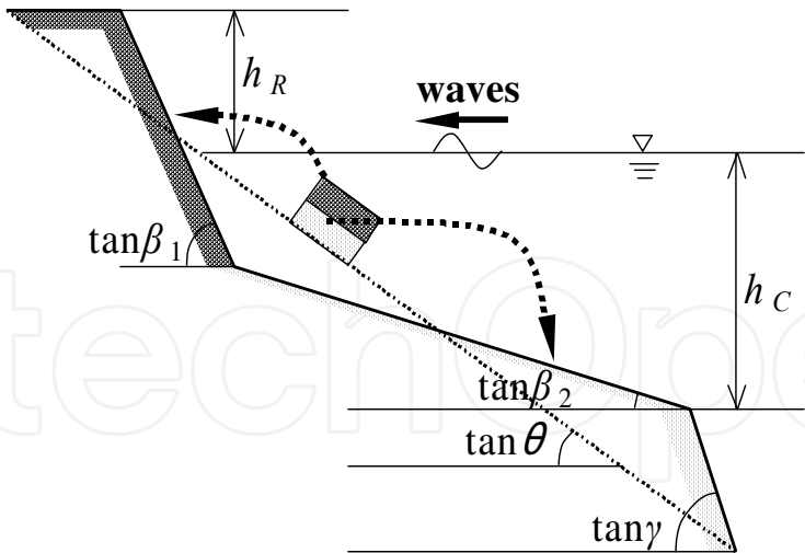
Fig. 2. Schematic diagram of concept of equilibrium slope corresponding to each grain size
