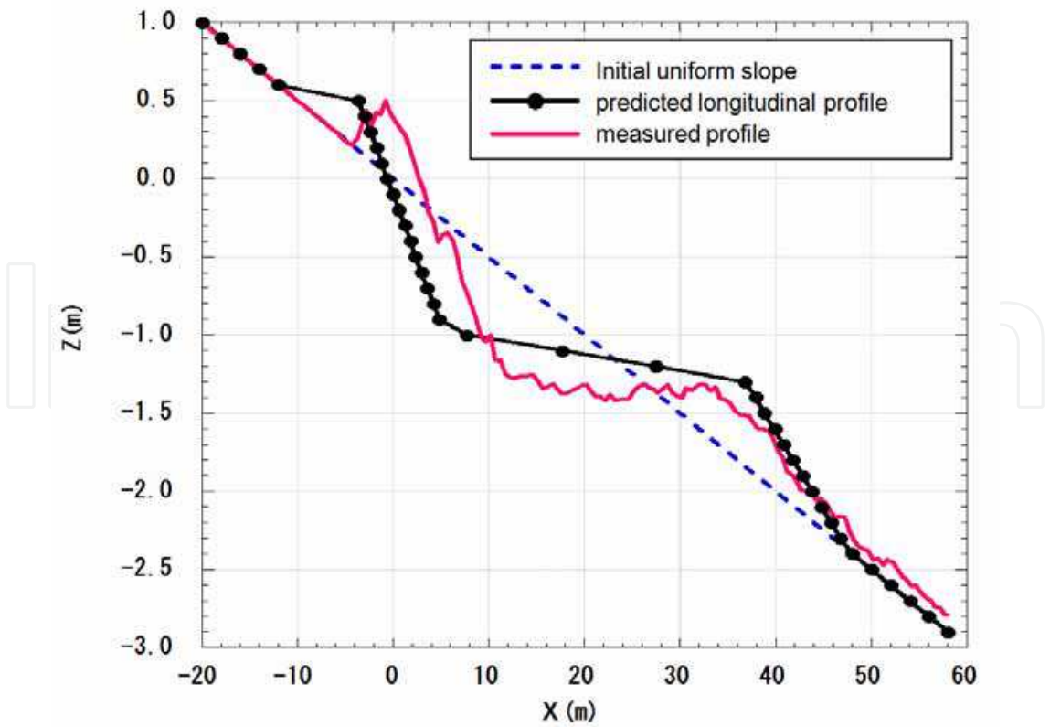
Fig. 6. Measured and predicted longitudinal profiles after wave action
