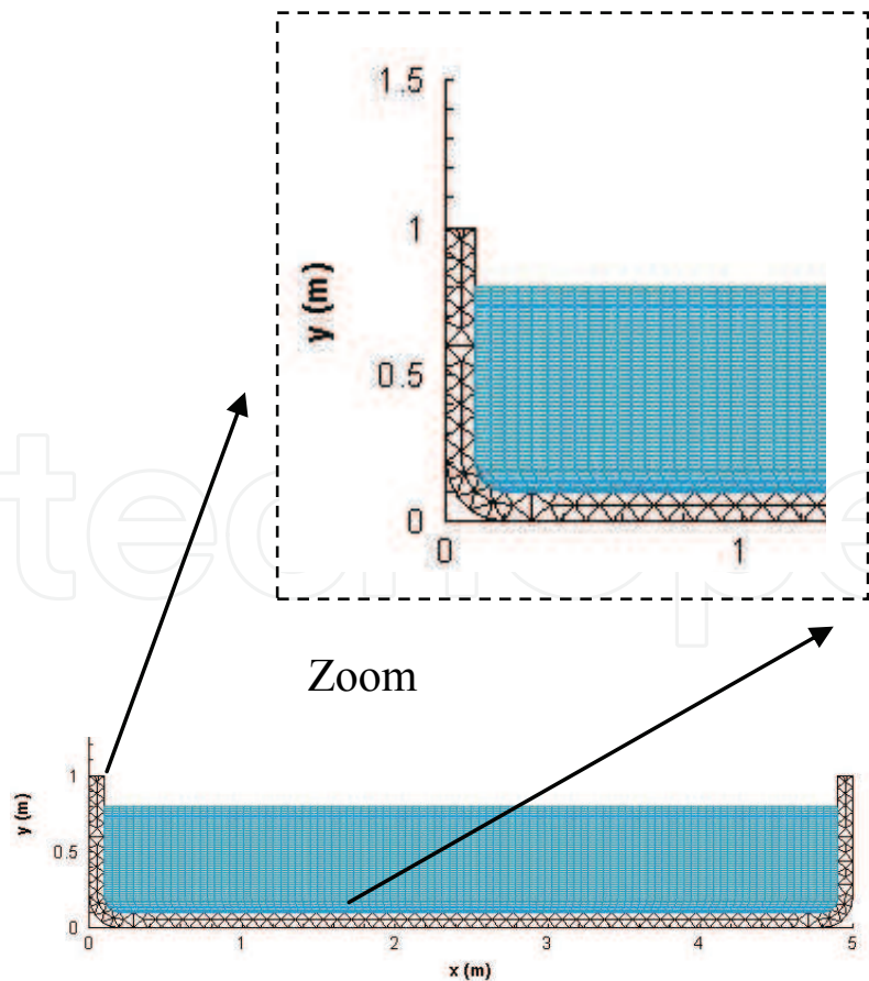
Fig. 7. The computational grid for the structure-flow in the case of \text{LO}_2 test case
