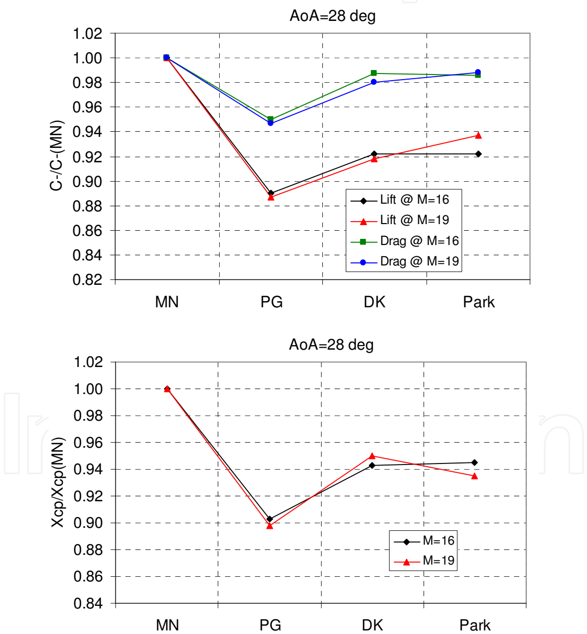
Fig. 20. Effect of chemical reactions on CRV aerodynamics at \alpha= 28 deg for M_\infty=16 and M_\infty=19 . Comparison among MN, PG, Dunn-Kang and Park computations
