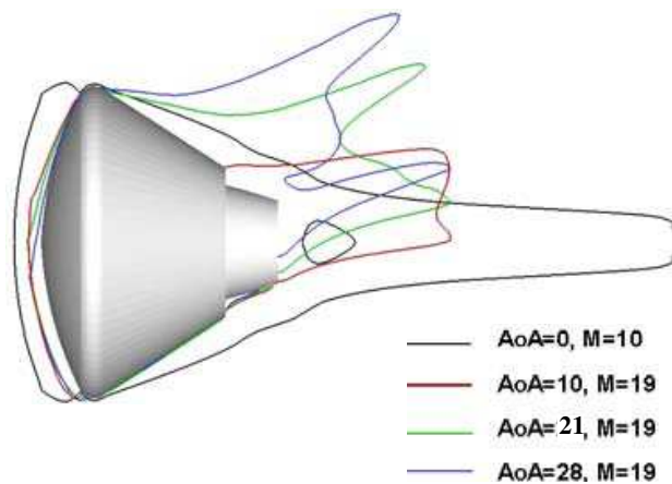
Fig. 15. Sonic line location in the capsule pitch plane for different AoA and Mach number
