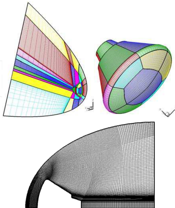
Fig. 3. Close-up view of 3-D (on top) and 2-D axis-symmetric computational mesh domains
