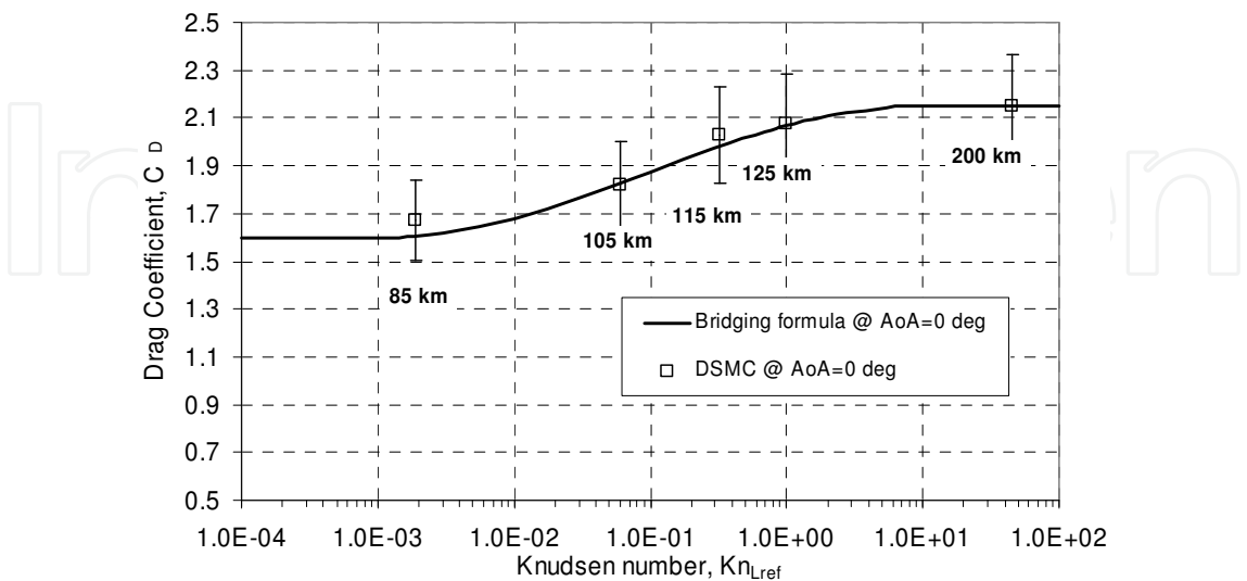
Fig. 22. Drag coefficients vs Knudsen number for \alpha=0 deg (Pezzella et al., 2009)
