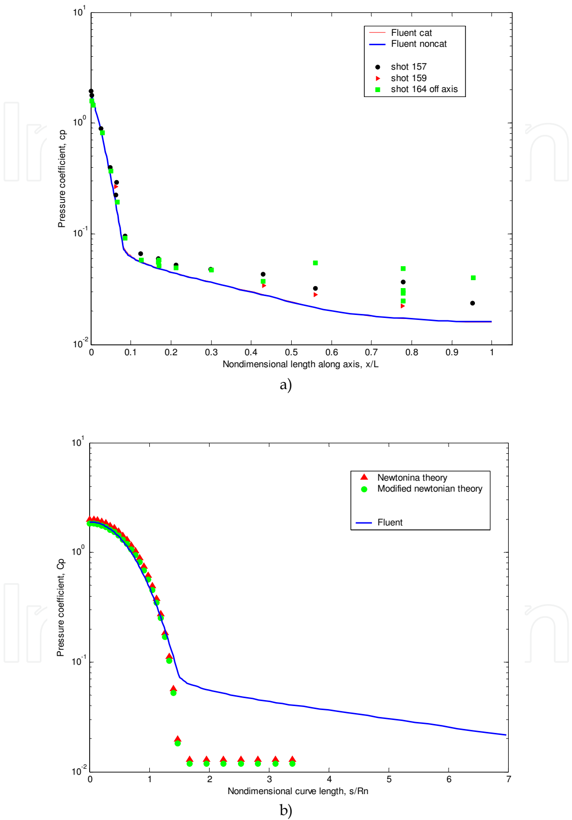
Fig. 6. a) C_p comparison between numerical, engineering, and experimental data, b) detail on the nose probe (Muylaert et al., 1999)
