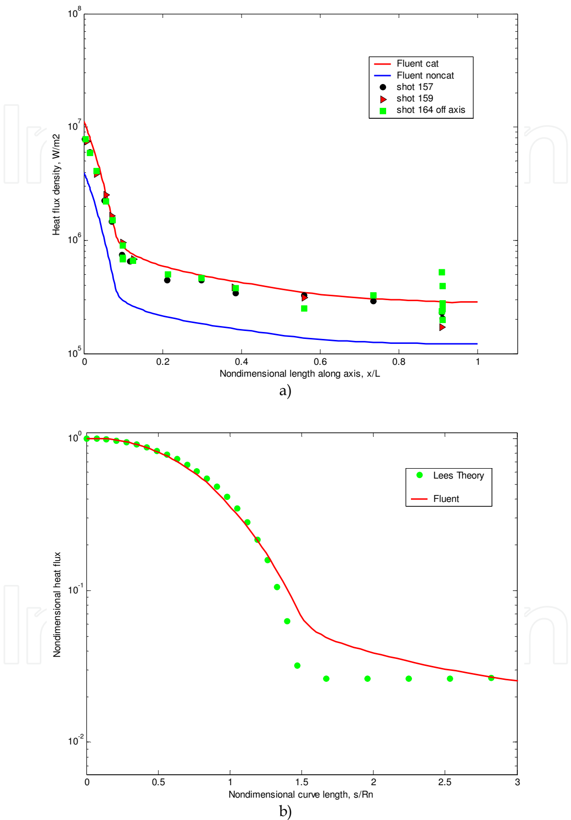
Fig. 7. Heat flux; a) comparison between numerical, engineering, and experimental data; b) detail on the nose probe (Muylaert et al., 1999)
