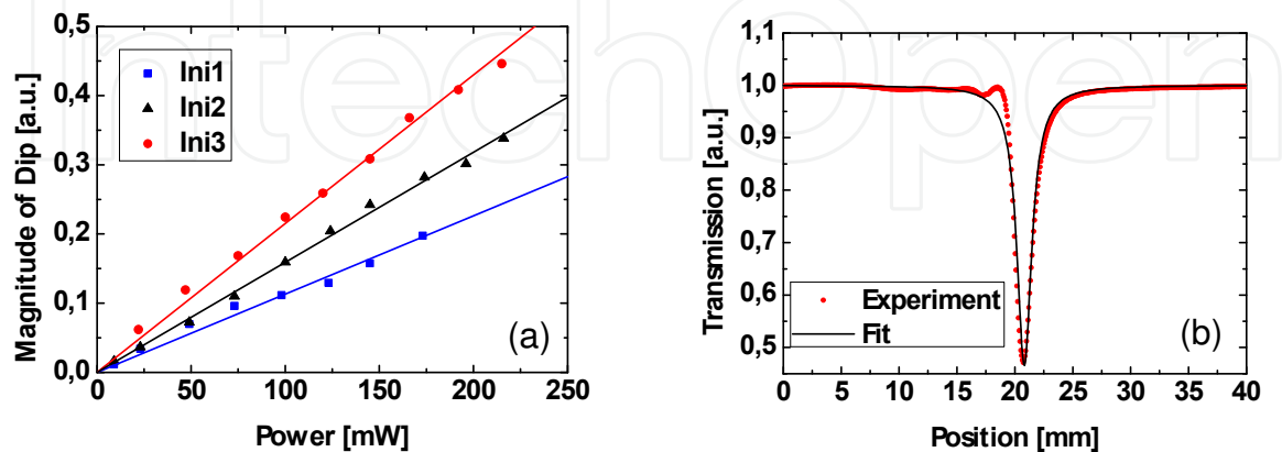
Fig. 6. z-scan results. (a) Magnitude of the transmission signal dip as a function of excitation power for three different photoinitiators. (b) Open aperture trace for Ini3 (for better illustration, only every fifth point is shown).
