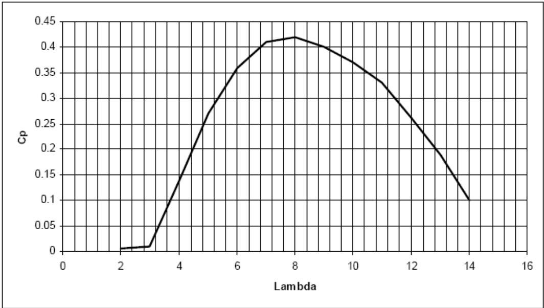
Fig. 7. Power coefficient C_p curve versus \lambda
