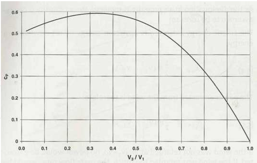
Fig. 6. Power coefficients C_p versus V_3/V_1 ratio
