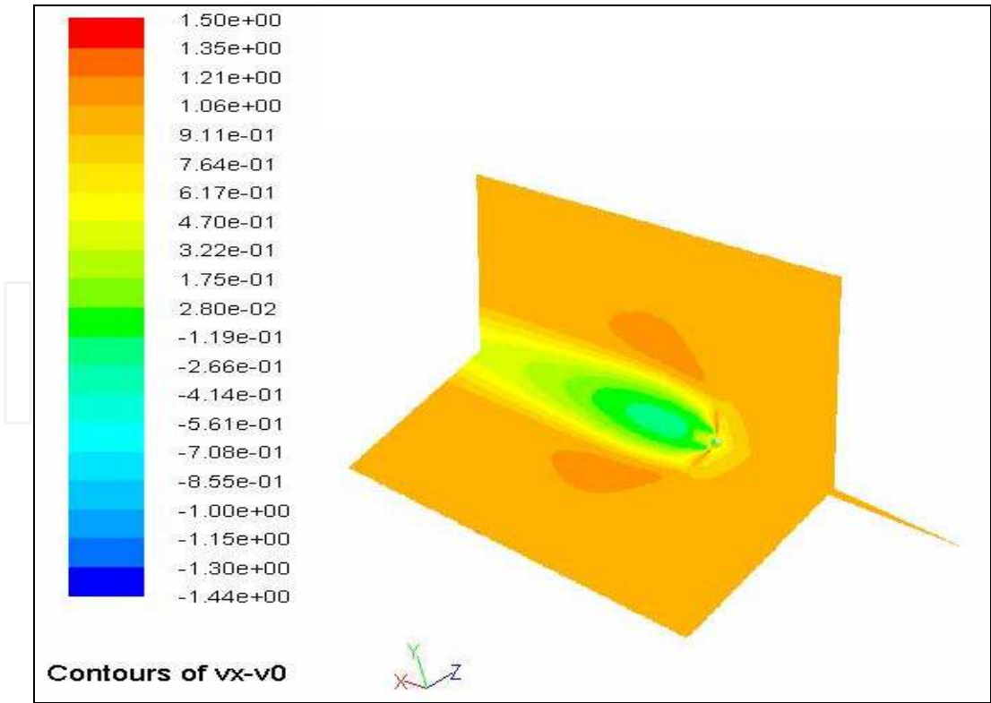
Fig. 12. Wake expansion along the flow at y = 0 inclined plane, which cuts through the turbine blade at angle of 60^\circ to the z -axis.
