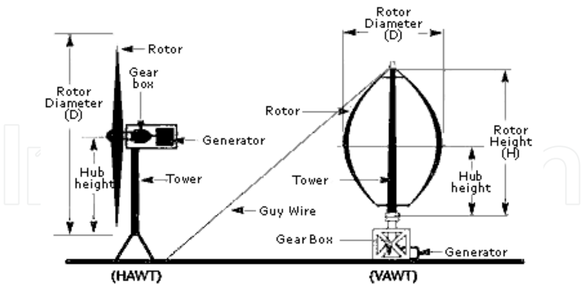
Fig. 2. Horizontal and vertical wind turbines
