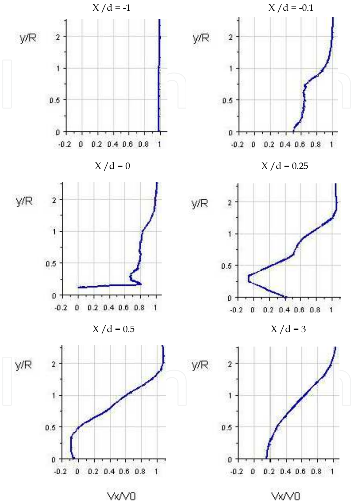
Fig. 13. Normalized axial velocity ( V_x/V_0 ) plots along the flow direction
