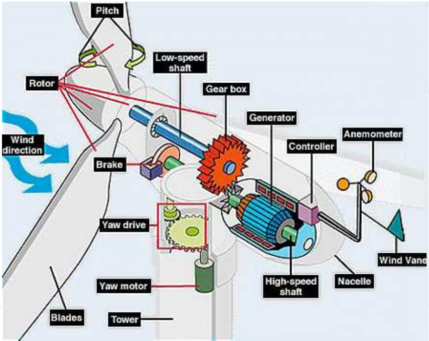
Fig. 3. Wind turbine parts
