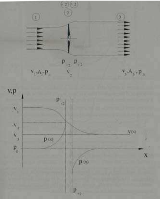
Fig. 5. Velocity and pressure distribution
